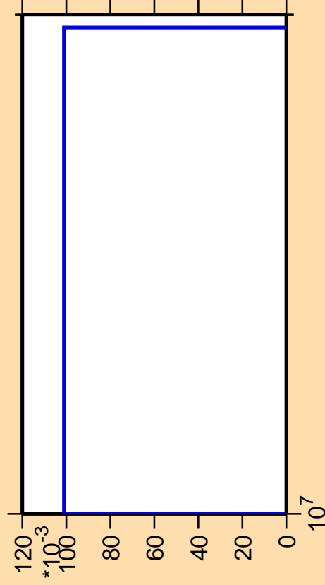
\Delta\sigma/\sigma vs. E for ^{103}\text{Nb}(n,2n\alpha)
