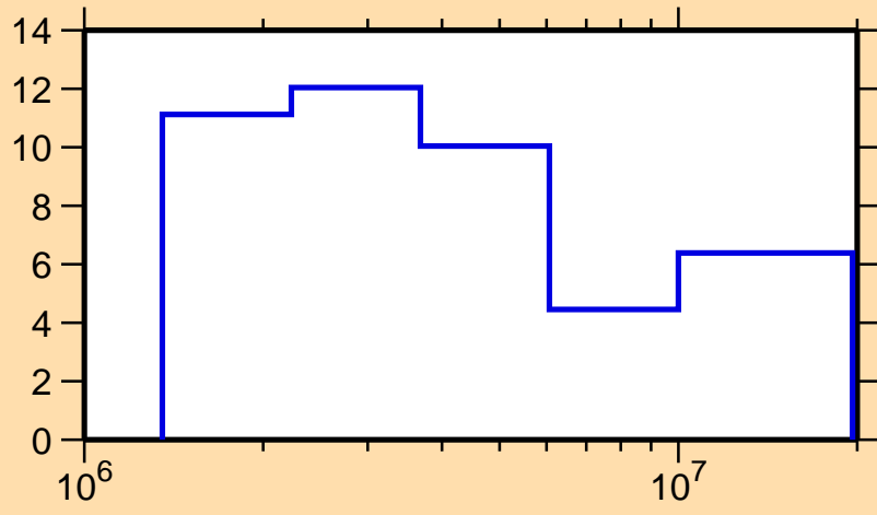
\Delta\sigma/\sigma vs. E for ^{103}\text{Nb}(n,\text{tot.})
