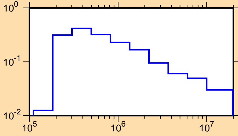
\sigma vs. E for ^{103}\text{Nb}(n,n_2)
