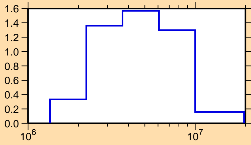
\sigma vs. E for ^{103}\text{Nb}(n,n\text{cont.})
