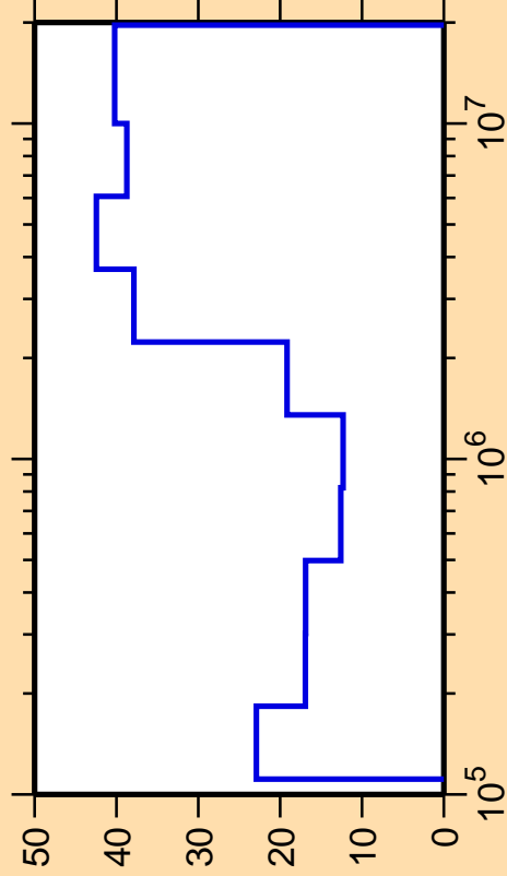
\Delta\sigma/\sigma vs. E for ^{103}\text{Nb}(n,n_2)
