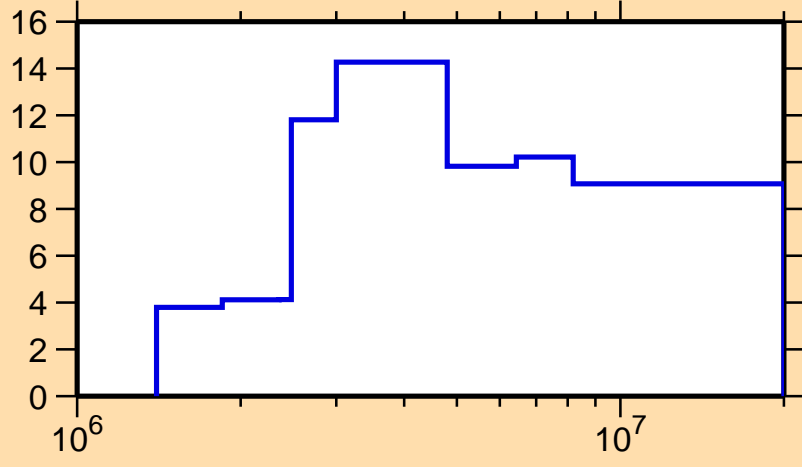
\Delta\sigma/\sigma vs. E for ^{103}\text{Nb}(n,n\text{onel.})
