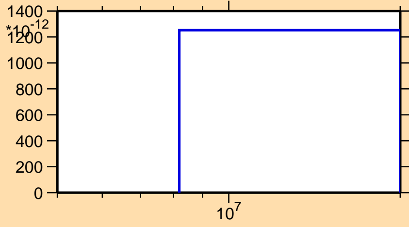
\sigma vs. E for ^{103}\text{Nb}(n,nd)
