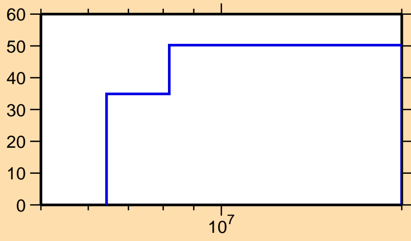
\Delta\sigma/\sigma vs. E for ^{103}\text{Nb}(n,ncont.)
