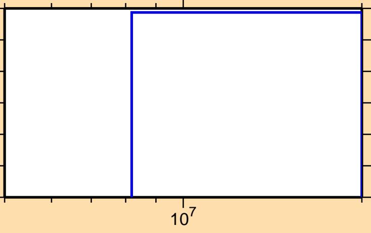
\sigma vs. E for ^{103}\text{Nb}(n,np)
