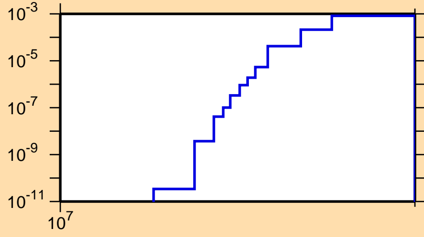
\sigma vs. E for ^{104}\text{Nb}(n,np)
