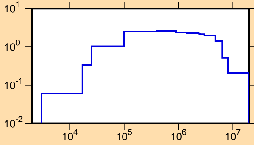
\sigma vs. E for ^{104}\text{Nb}(n,\text{inel.})
