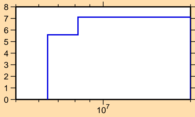
\Delta\sigma/\sigma vs. E for ^{104}\text{Nb}(n,\text{tot.})
