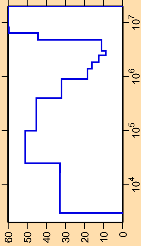
\Delta\sigma/\sigma vs. E for ^{104}\text{Nb}(n,\text{inel.})
