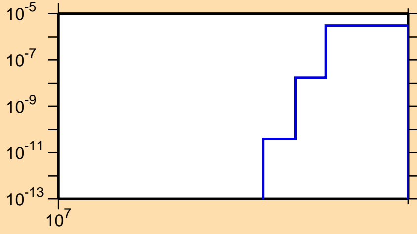
\sigma vs. E for ^{105}\text{Nb}(n,nt)
