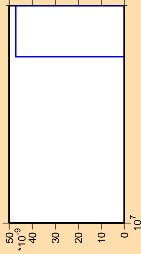
\Delta\sigma/\sigma vs. E for ^{105}\text{Nb} (mt 11)
