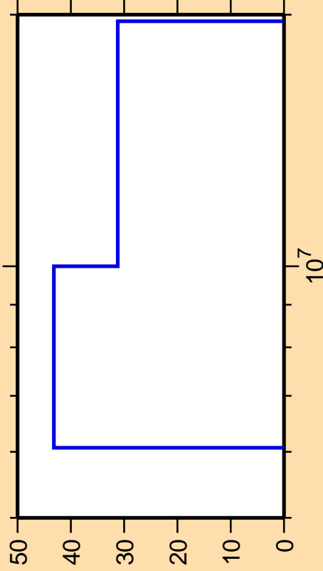
\Delta\sigma/\sigma vs. E for ^{105}\text{Nb}(n,p)
