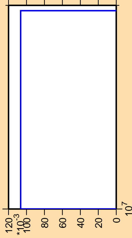
\Delta\sigma/\sigma vs. E for ^{105}\text{Nb}(n,2np)
