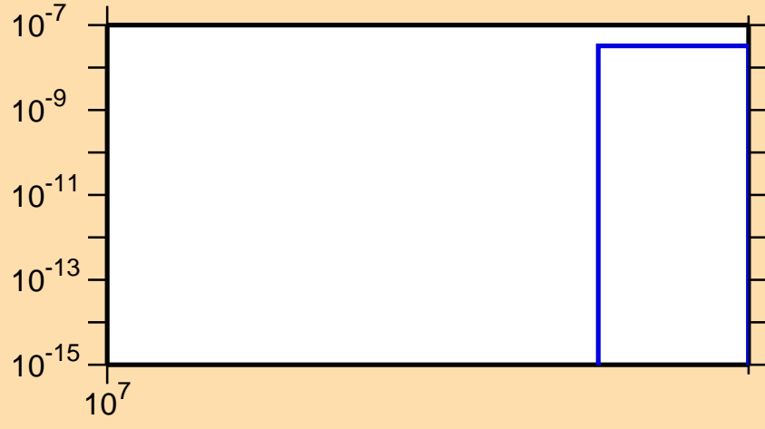
\sigma vs. E for ^{106}\text{Nb}(n,2np)
