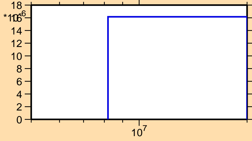
\sigma vs. E for ^{106}\text{Nb}(n,t)
