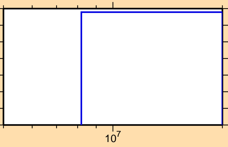
\sigma vs. E for ^{106}\text{Nb}(n,\text{nd})
