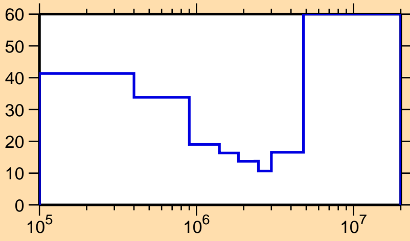
\Delta\sigma/\sigma vs. E for ^{106}\text{Nb}(n,n\text{cont.})
