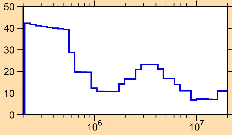
\Delta\sigma/\sigma vs. E for ^{126}\text{Nd}(n,\text{el.})
