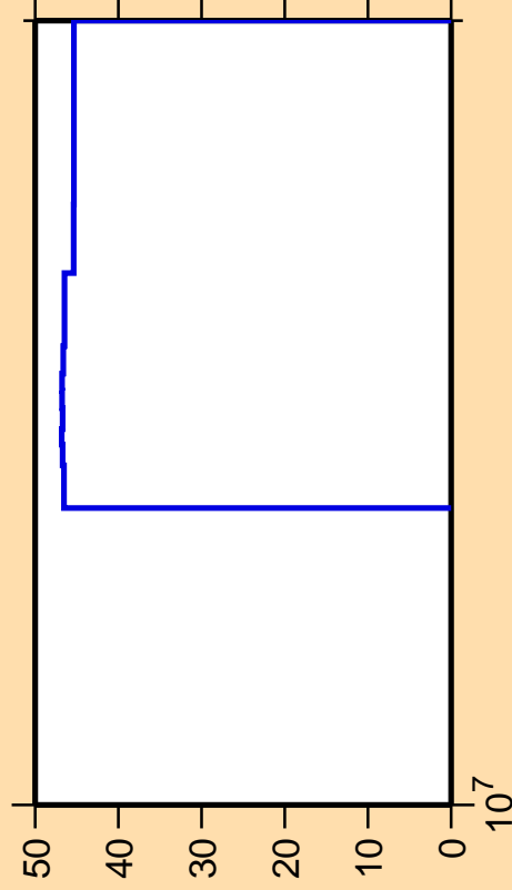
\Delta\sigma/\sigma vs. E for ^{126}\text{Nd}(n,n\text{cont.})
