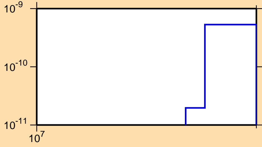
\sigma vs. E for ^{126}\text{Nd} (mt 34)
