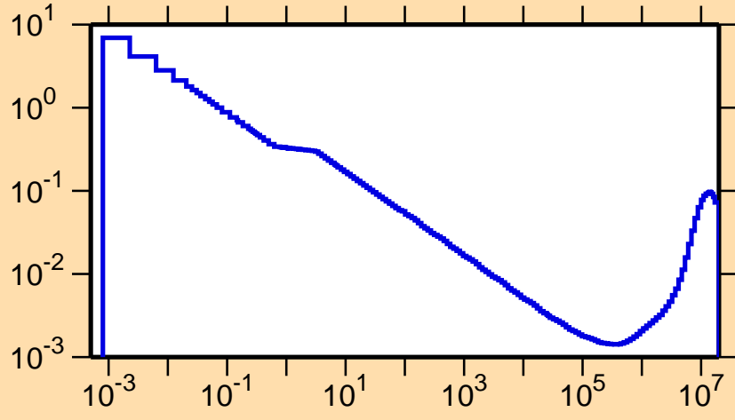
\sigma vs. E for ^{126}\text{Nd}(n,\alpha)
