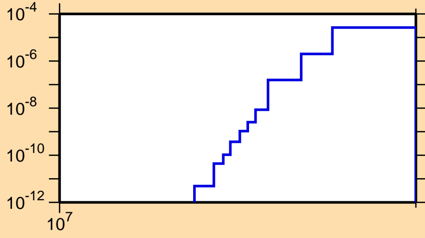
\sigma vs. E for ^{126}\text{Nd}(n,\text{pt})
