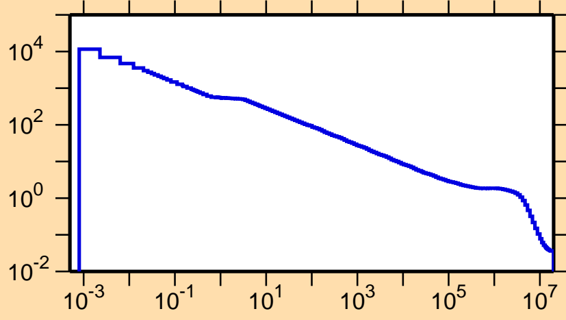
\sigma vs. E for ^{126}\text{Nd}(n,p)
