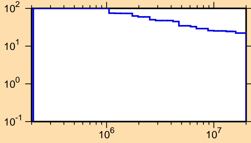
\Delta\sigma/\sigma vs. E for ^{126}\text{Nd}(n,\text{inel.})
