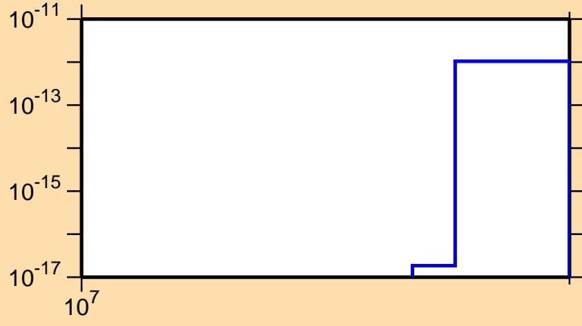
\sigma vs. E for ^{126}\text{Nd}(n,2n\alpha)
