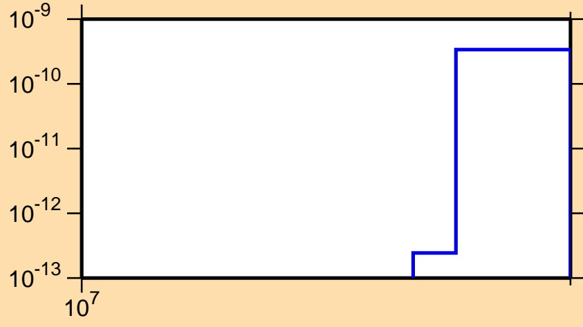
\sigma vs. E for ^{126}\text{Nd}(n,\text{nd})
