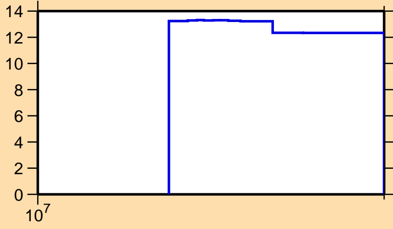
\Delta\sigma/\sigma vs. E for ^{126}\text{Nd}(n,\text{nonel.})
