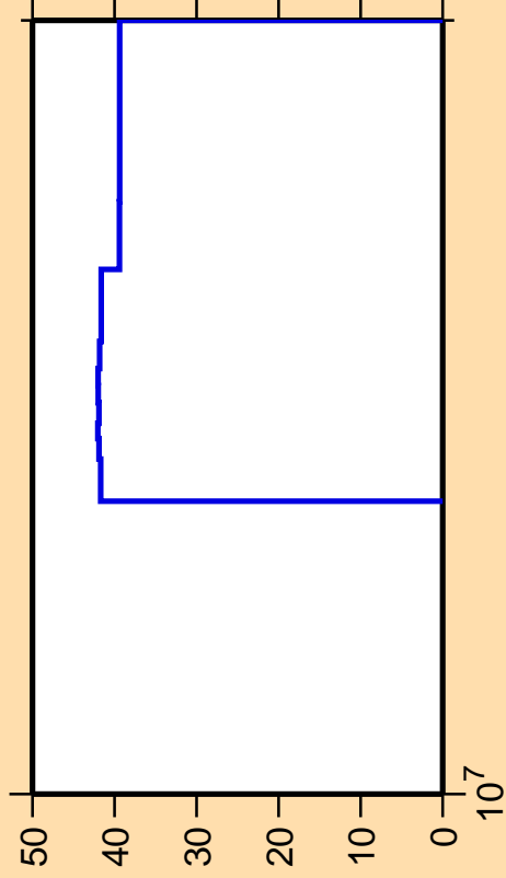
\Delta\sigma/\sigma vs. E for ^{126}\text{Nd}(n,n_1)
