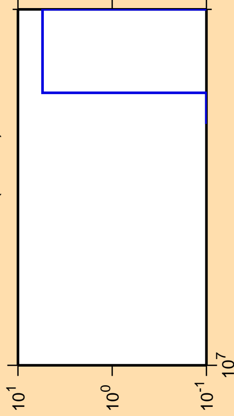
\Delta\sigma/\sigma vs. E for ^{126}\text{Nd}(n,2n\alpha)
