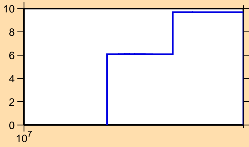
\Delta\sigma/\sigma vs. E for ^{126}\text{Nd}(n,\text{tot.})
