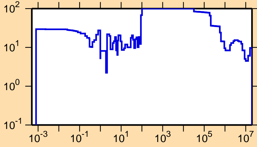
\Delta\sigma/\sigma vs. E for ^{126}\text{Nd}(n,\text{tot.})
