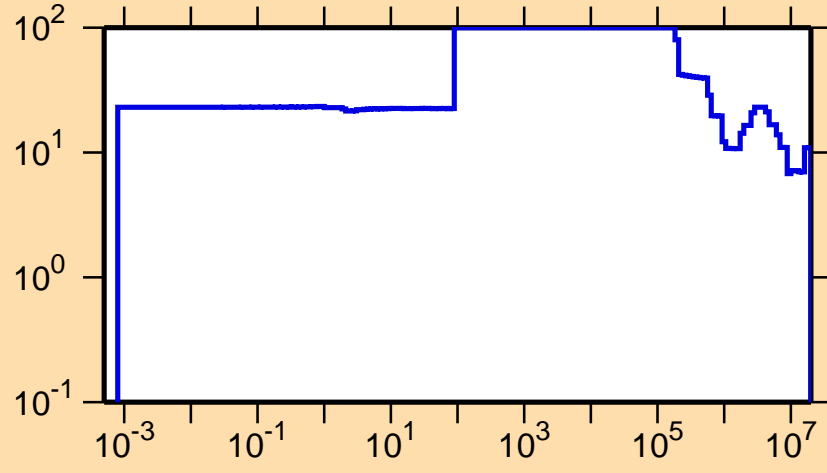
\Delta\sigma/\sigma vs. E for ^{126}\text{Nd}(n,\text{el.})
