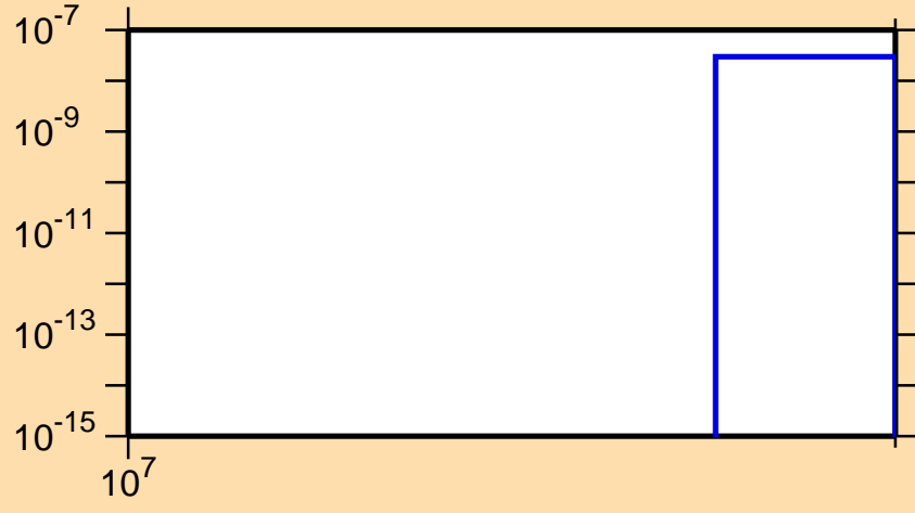
\sigma vs. E for ^{126}\text{Nd}(n,2np)
