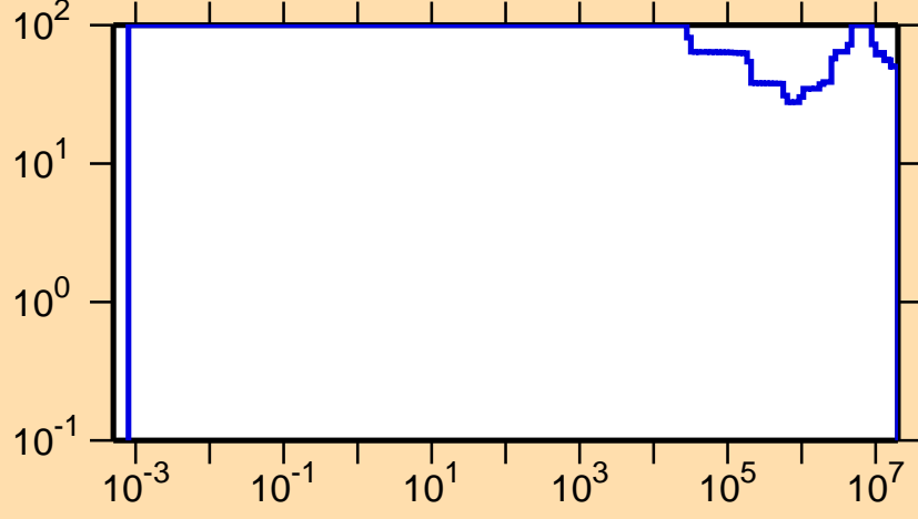
\Delta\sigma/\sigma vs. E for ^{126}\text{Nd}(n,p)
