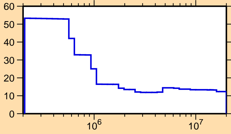
\Delta\sigma/\sigma vs. E for ^{126}\text{Nd}(n,\text{nonel.})
