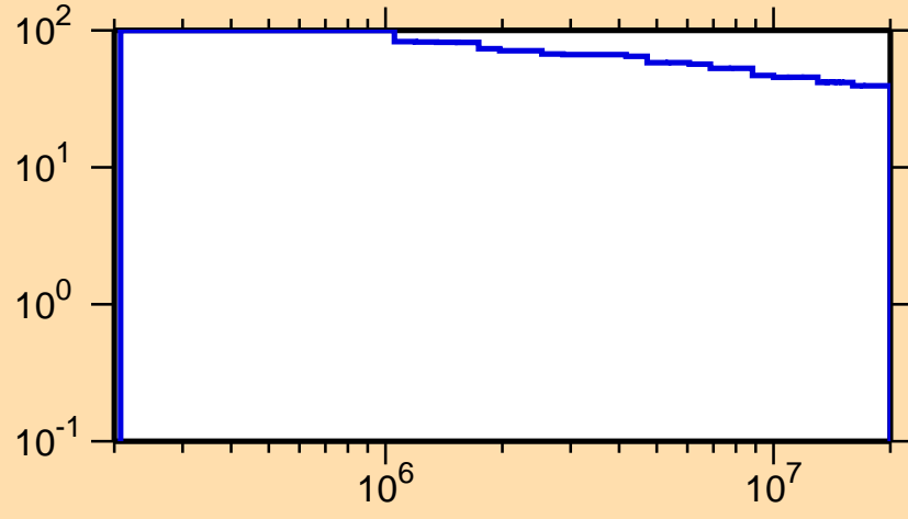
\Delta\sigma/\sigma vs. E for ^{126}\text{Nd}(n,n_1)
