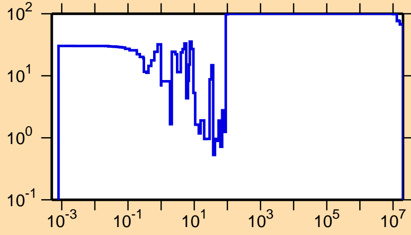
\Delta\sigma/\sigma vs. E for ^{126}\text{Nd}(n,\gamma)
