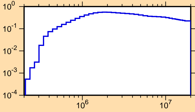
\sigma vs. E for ^{126}\text{Nd}(n,\text{inel.})
