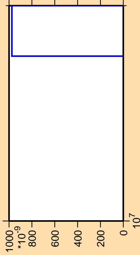
\Delta\sigma/\sigma vs. E for ^{126}\text{Nd}(n,nt)
