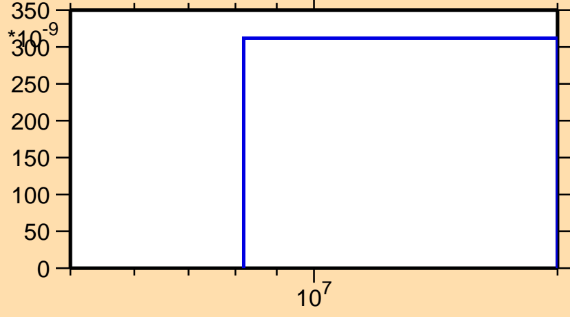
\sigma vs. E for ^{126}\text{Nd}(n,\text{pt})
