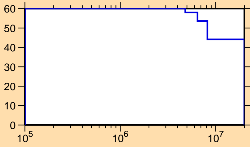
\Delta\sigma/\sigma vs. E for ^{126}\text{Nd}(n,n_1)
