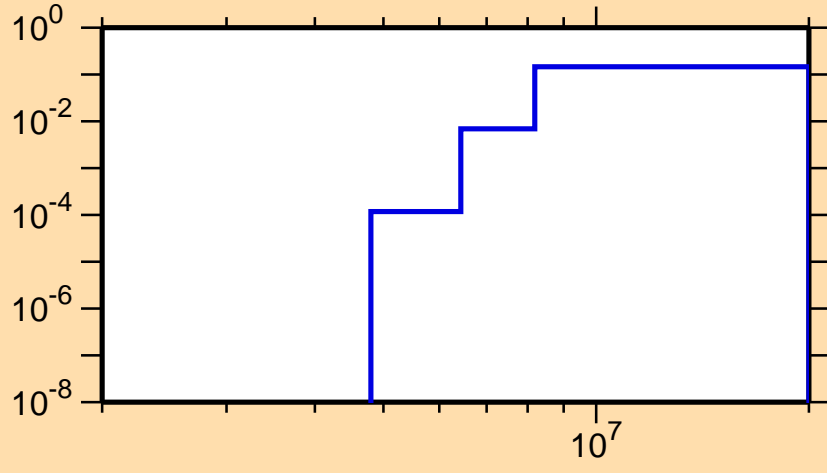
\sigma vs. E for ^{126}\text{Nd}(n,np)
