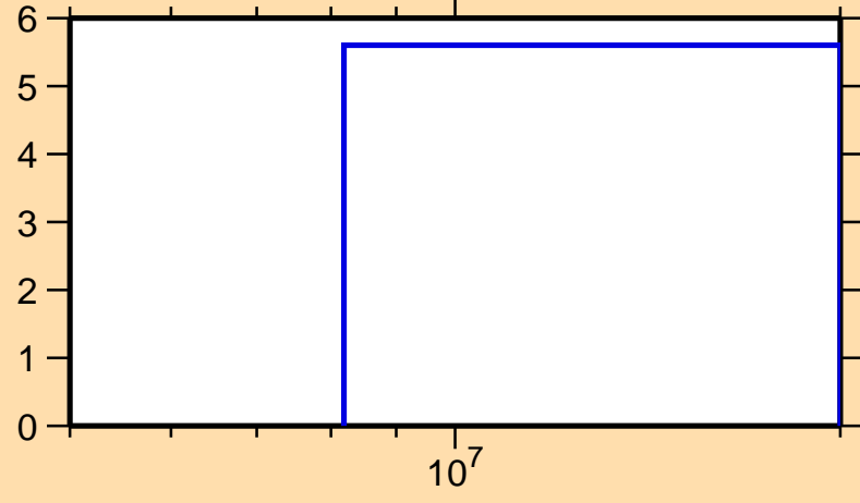
\Delta\sigma/\sigma vs. E for ^{126}\text{Nd}(n,\text{tot.})
