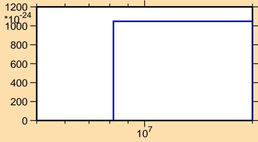
\sigma vs. E for ^{126}\text{Nd}(n,nt)
