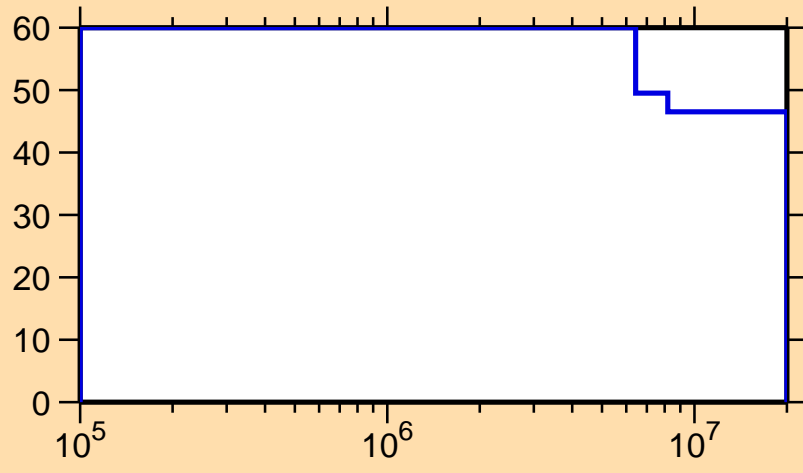
\Delta\sigma/\sigma vs. E for ^{126}\text{Nd}(n,n\text{cont.})
