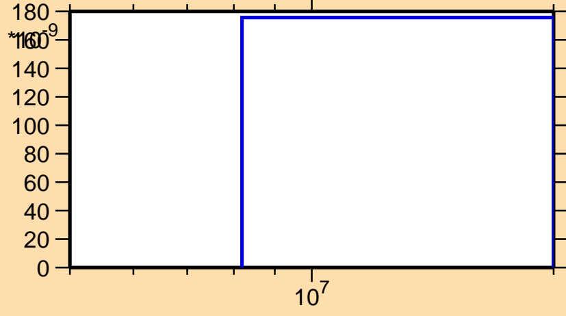
\sigma vs. E for ^{126}\text{Nd}(\text{mt } 45)
