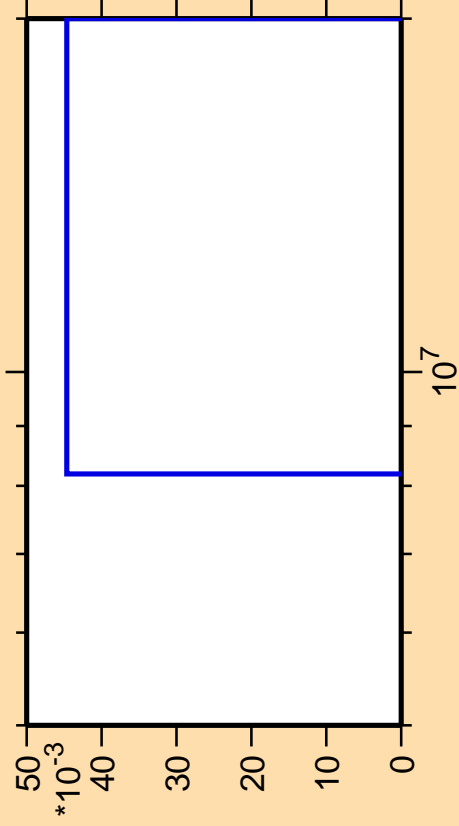
\Delta\sigma/\sigma vs. E for ^{126}\text{Nd}(n,2n\alpha)
