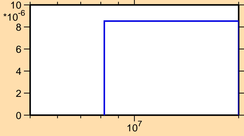
\sigma vs. E for ^{126}\text{Nd}(n,2n)
