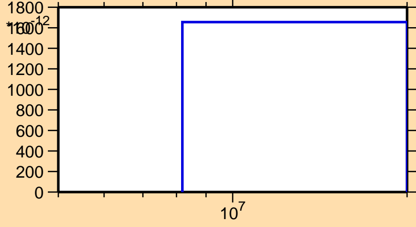
\sigma vs. E for ^{126}\text{Nd}(\text{mt117})
