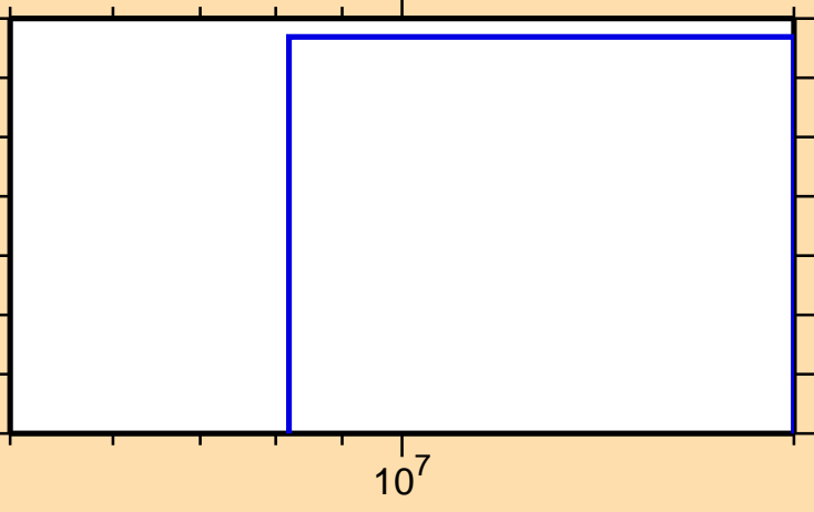
\sigma vs. E for ^{126}\text{Nd}(n,t)
