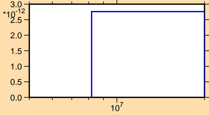
\sigma vs. E for ^{126}\text{Nd}(n,\text{nd})
