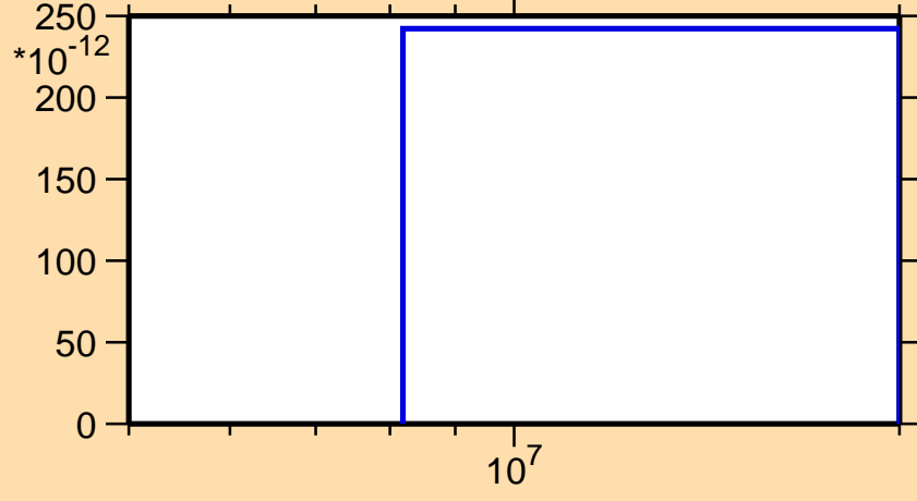
\sigma vs. E for ^{126}\text{Nd}(n,2np)
