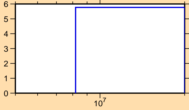
\Delta\sigma/\sigma vs. E for ^{126}\text{Nd}(n,\text{el.})
