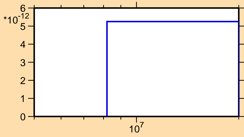
\sigma vs. E for ^{126}\text{Nd}(\text{mt } 34)
