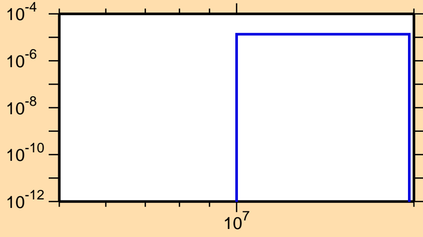
\sigma vs. E for ^{127}\text{Nd}(n,\text{pt})
