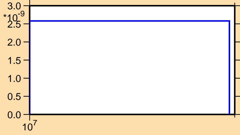
\sigma vs. E for ^{127}\text{Nd} (mt 34)
