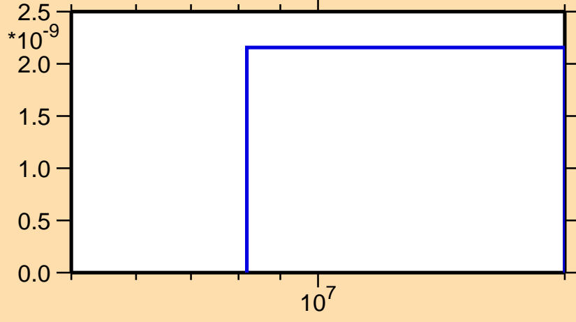
\sigma vs. E for ^{127}\text{Nd}(\text{mt } 34)
