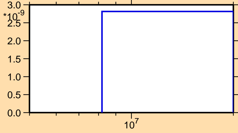
\sigma vs. E for ^{127}\text{Nd}(n,\text{nd})
