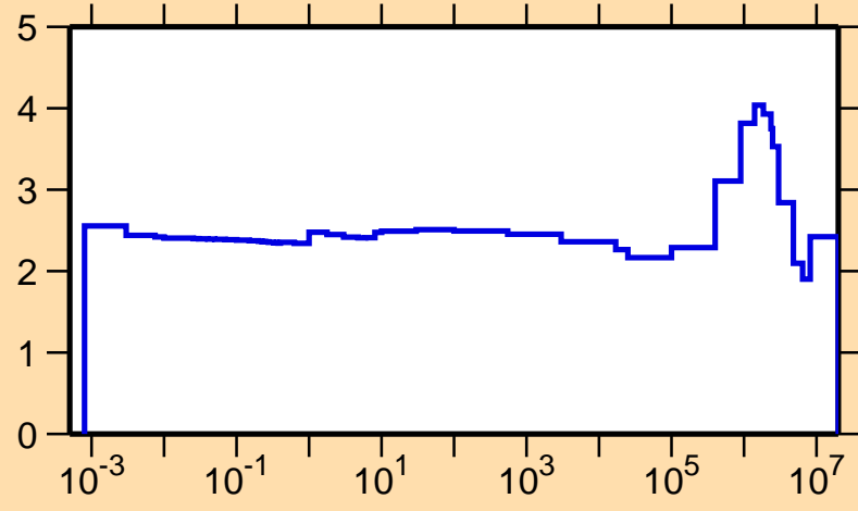
\sigma vs. E for ^{127}\text{Nd}(n,\text{el.})
