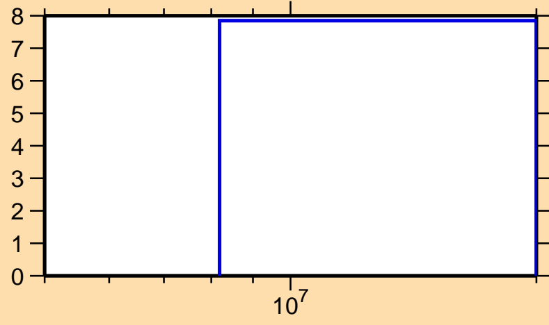
\Delta\sigma/\sigma vs. E for ^{127}\text{Nd}(n,\text{el.})
