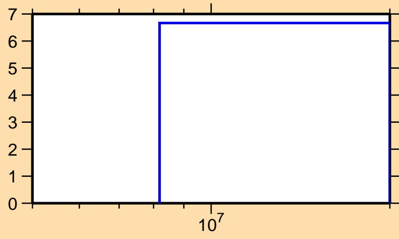
\Delta\sigma/\sigma vs. E for ^{127}\text{Nd}(n,\text{tot.})
