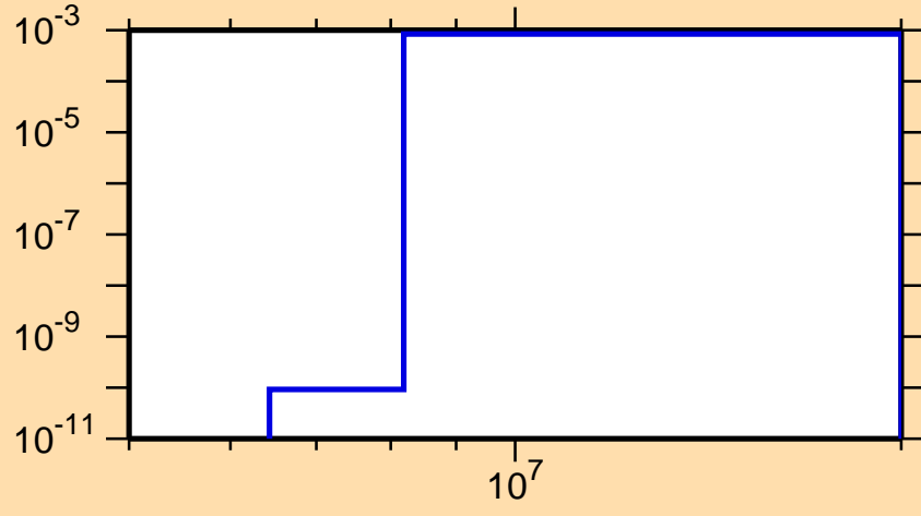
\sigma vs. E for ^{127}\text{Nd}(n,\text{pd})
