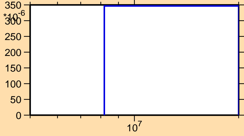
\sigma vs. E for ^{127}\text{Nd}(n,2n)
