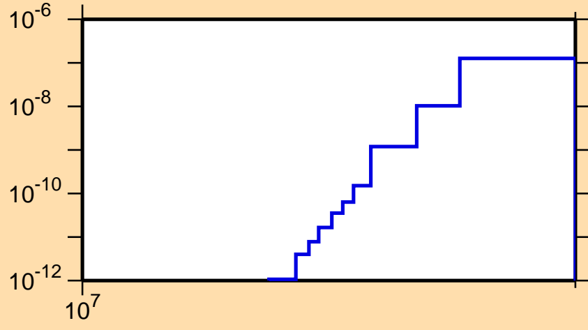
\sigma vs. E for ^{129}\text{Nd}(\text{mt } 34)
