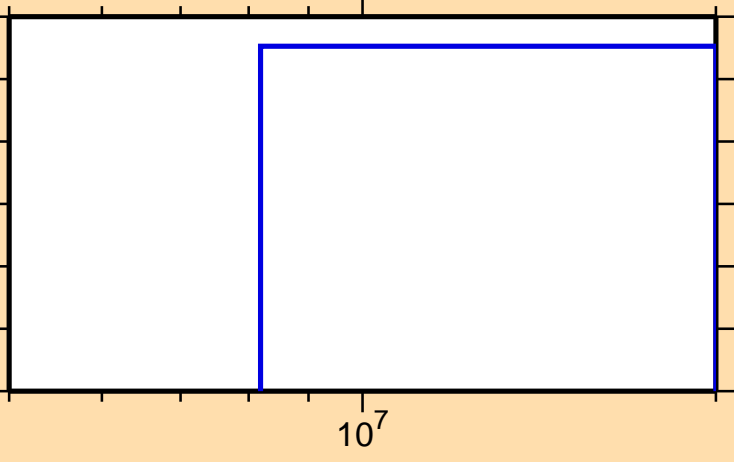
\sigma vs. E for ^{129}\text{Nd}(\text{mt } 45)
