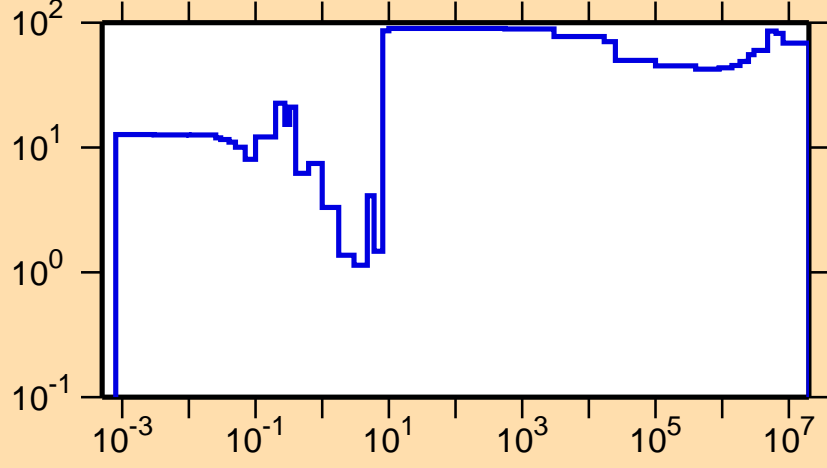
\Delta\sigma/\sigma vs. E for ^{129}\text{Nd}(n,\gamma)
