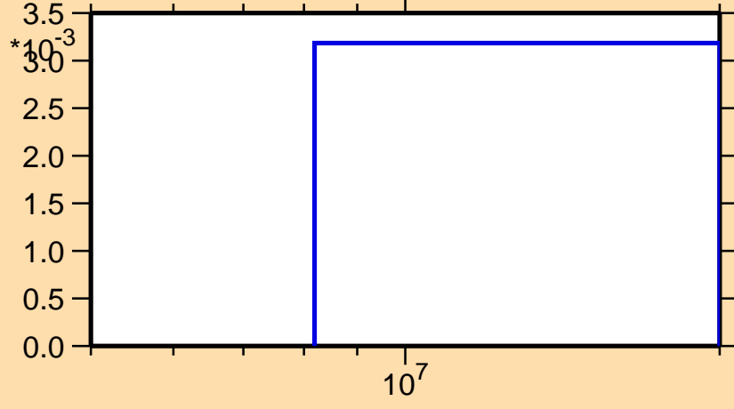
\sigma vs. E for ^{129}\text{Nd}(n,2n)
