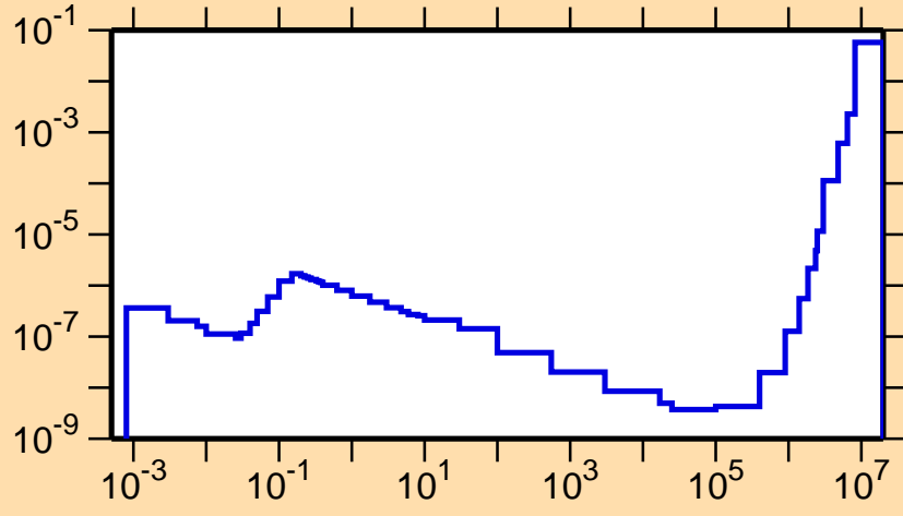
\sigma vs. E for ^{129}\text{Nd}(n,p\alpha)
