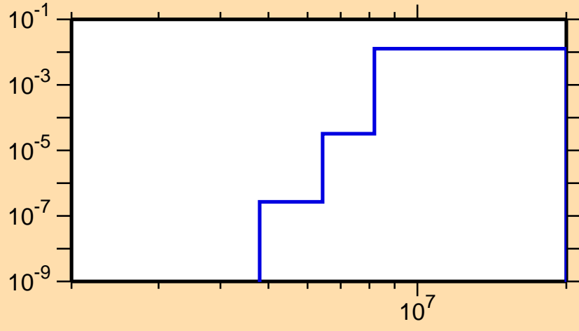
\sigma vs. E for ^{129}\text{Nd}(n,d)
