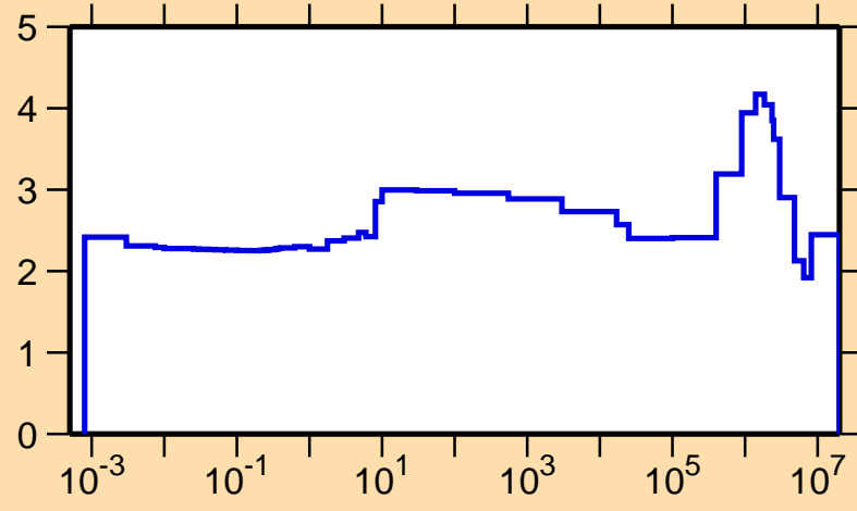
\sigma vs. E for ^{129}\text{Nd}(n,\text{el.})
