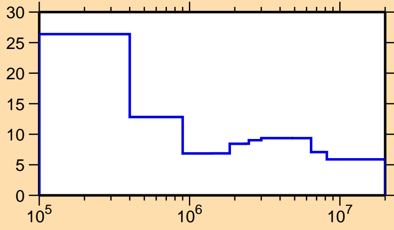
\Delta\sigma/\sigma vs. E for ^{129}\text{Nd}(n,\text{tot.})
