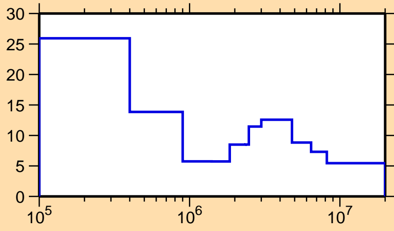
\Delta\sigma/\sigma vs. E for ^{129}\text{Nd}(n,\text{el.})
