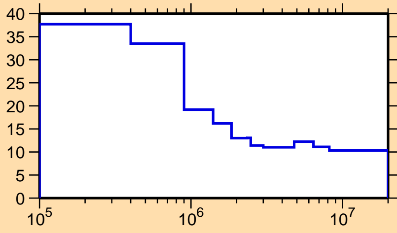
\Delta\sigma/\sigma vs. E for ^{129}\text{Nd}(n,\text{nonel.})
