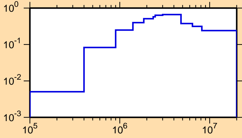
\sigma vs. E for ^{129}\text{Nd}(n,\text{inel.})
