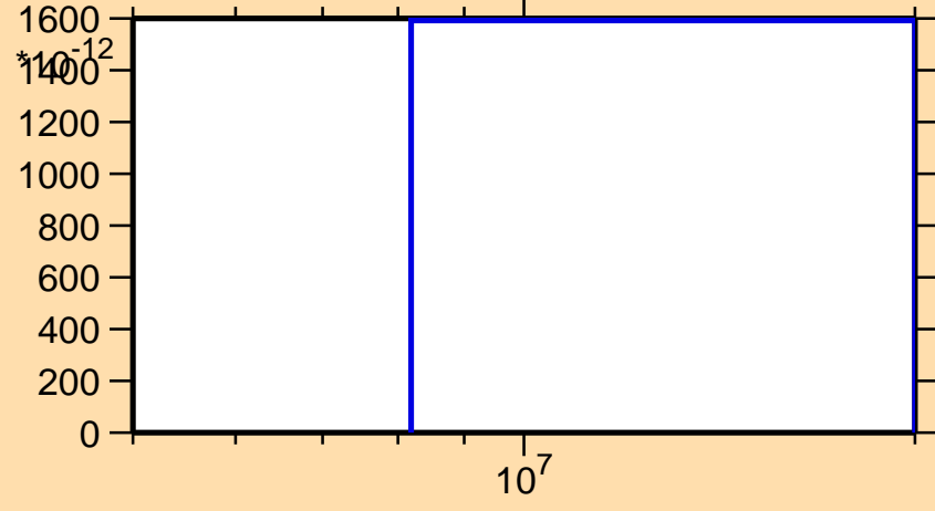
\sigma vs. E for ^{129}\text{Nd} (mt 34)
