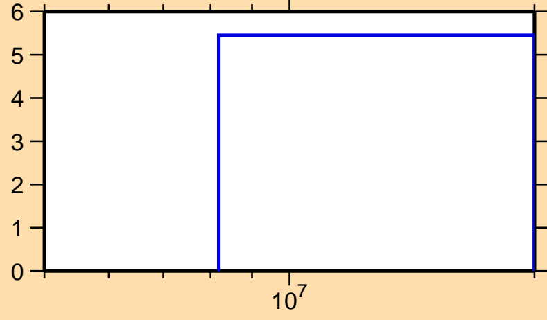
\Delta\sigma/\sigma vs. E for ^{129}\text{Nd}(n,\text{el.})
