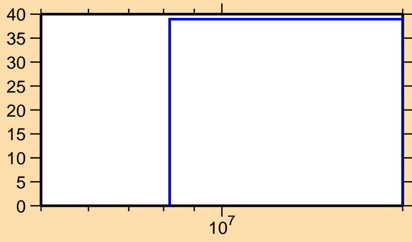
\Delta\sigma/\sigma vs. E for ^{129}\text{Nd}(n,\text{inel.})
