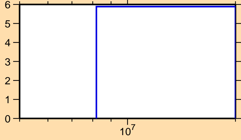
\Delta\sigma/\sigma vs. E for ^{129}\text{Nd}(n,\text{tot.})
