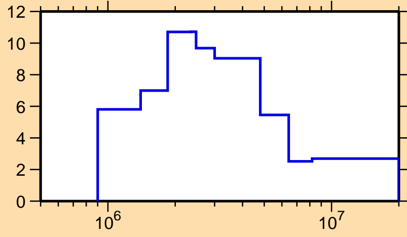
\Delta\sigma/\sigma vs. E for ^{130}\text{Nd}(n,\text{tot.})
