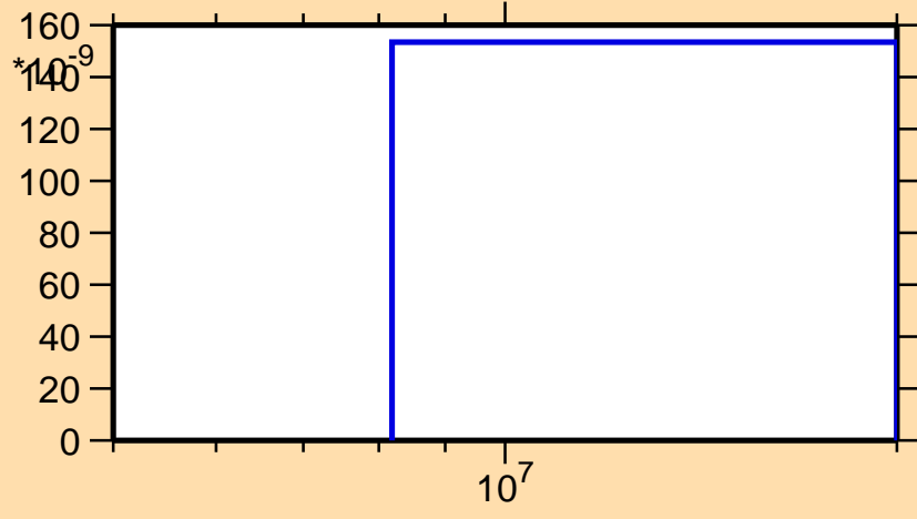
\sigma vs. E for ^{130}\text{Nd}(\text{mt } 45)
