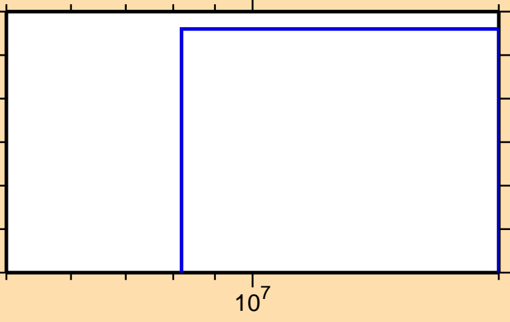
\sigma vs. E for ^{130}\text{Nd}(n,t)
