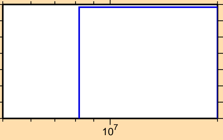
\sigma vs. E for ^{130}\text{Nd}(\text{mt117})
