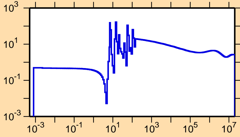
\sigma vs. E for ^{132}\text{Nd}(n,\text{el.})
