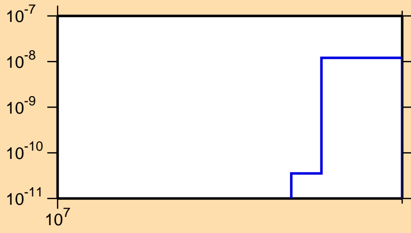
\sigma vs. E for ^{132}\text{Nd}(n,2n\alpha)
