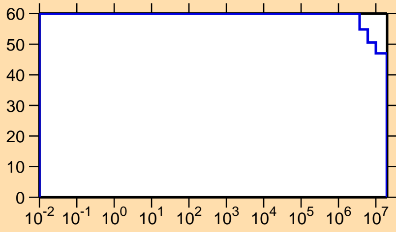
\Delta\sigma/\sigma vs. E for ^{132}\text{Nd}(n,p)
