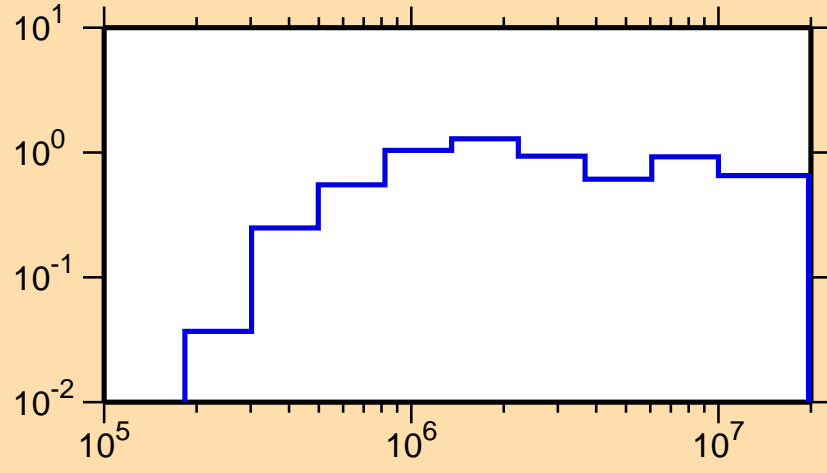
\sigma vs. E for ^{132}\text{Nd}(n,\text{inel.})
