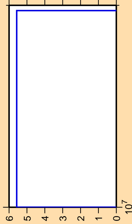
\Delta\sigma/\sigma vs. E for ^{132}\text{Nd} (mt 34)
