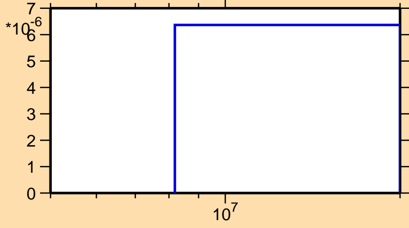
\sigma vs. E for ^{132}\text{Nd}(n,\text{pd})
