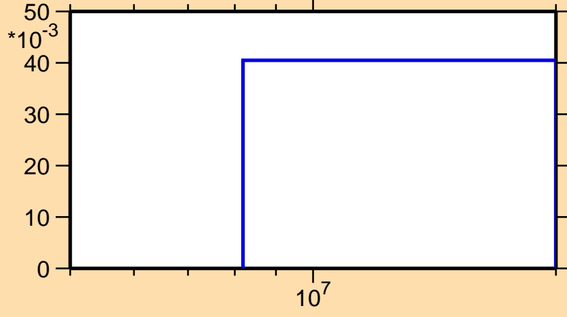
\sigma vs. E for ^{132}\text{Nd}(n,2n)
