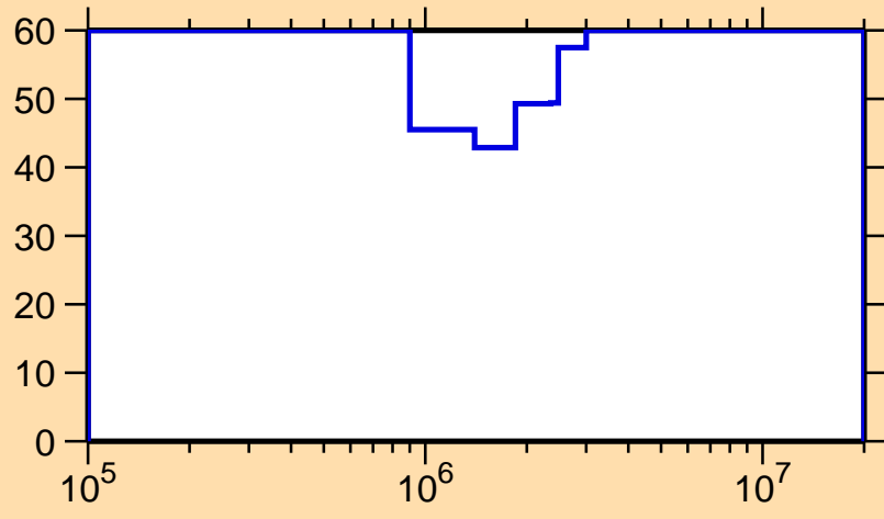
\Delta\sigma/\sigma vs. E for ^{132}\text{Nd}(n,n_1)
