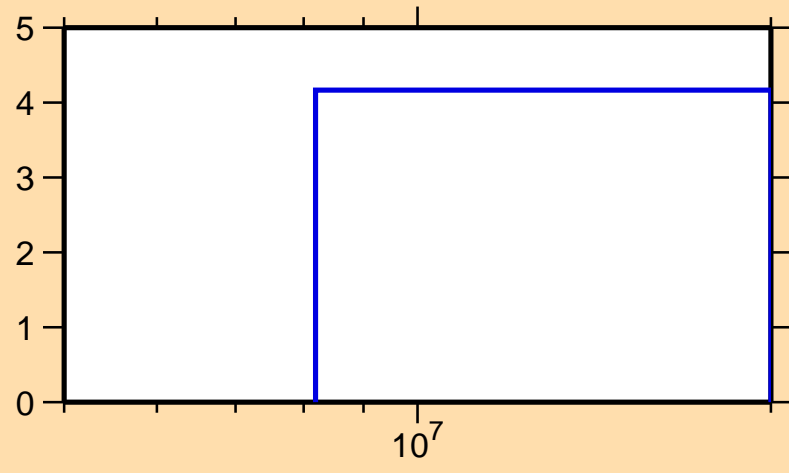
\Delta\sigma/\sigma vs. E for ^{132}\text{Nd}(n,\text{tot.})
