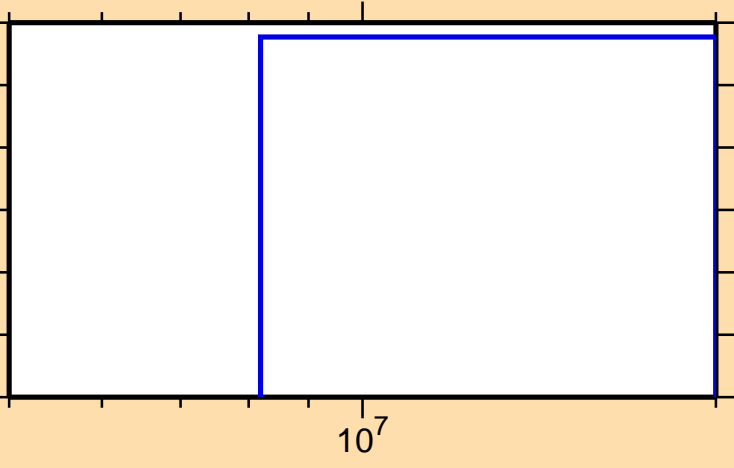
\sigma vs. E for ^{132}\text{Nd}(n,t)
