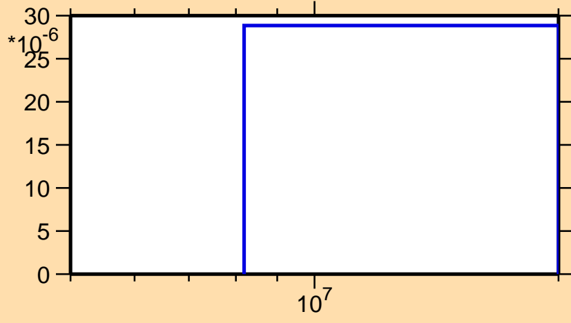
\sigma vs. E for ^{132}\text{Nd}(n,t)
