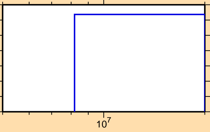
\sigma vs. E for ^{132}\text{Nd}(n,\text{pd})
