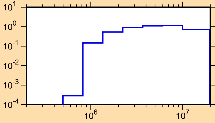
\sigma vs. E for ^{133}\text{Nd}(n,n\text{cont.})
