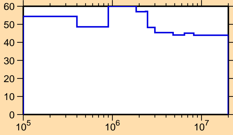
\Delta\sigma/\sigma vs. E for ^{133}\text{Nd}(n,n_1)
