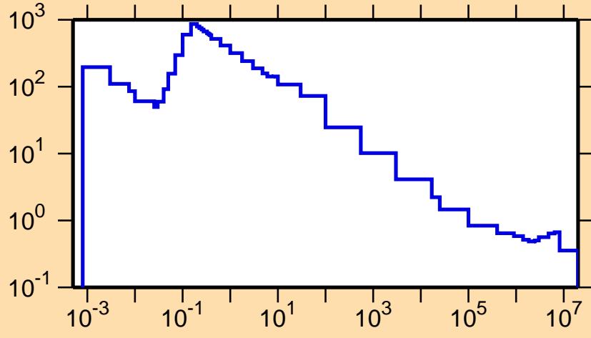
\sigma vs. E for ^{133}\text{Nd}(n,p)
