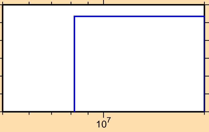
\sigma vs. E for ^{133}\text{Nd}(n,2np)
