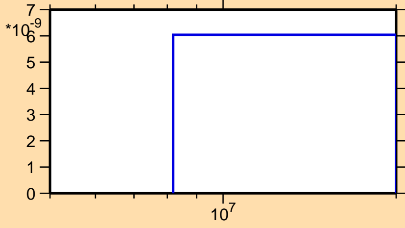
\sigma vs. E for ^{133}\text{Nd}(\text{mt } 45)
