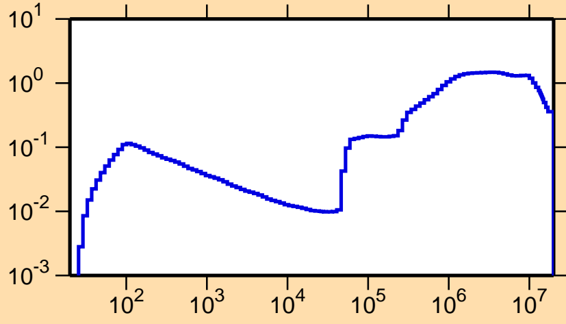
\sigma vs. E for ^{133}\text{Nd}(n,\text{inel.})
