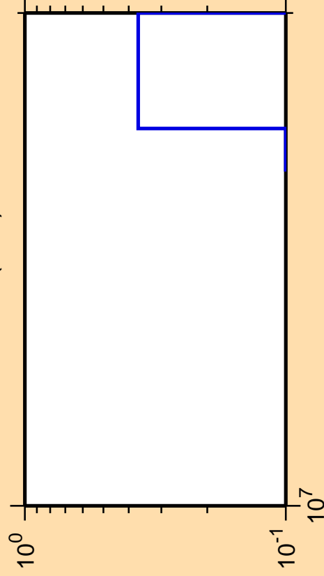
\Delta\sigma/\sigma vs. E for ^{133}\text{Nd}(n,nt)
