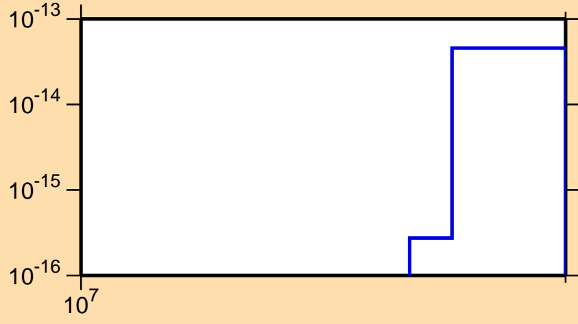
\sigma vs. E for ^{133}\text{Nd}(n,nt)
