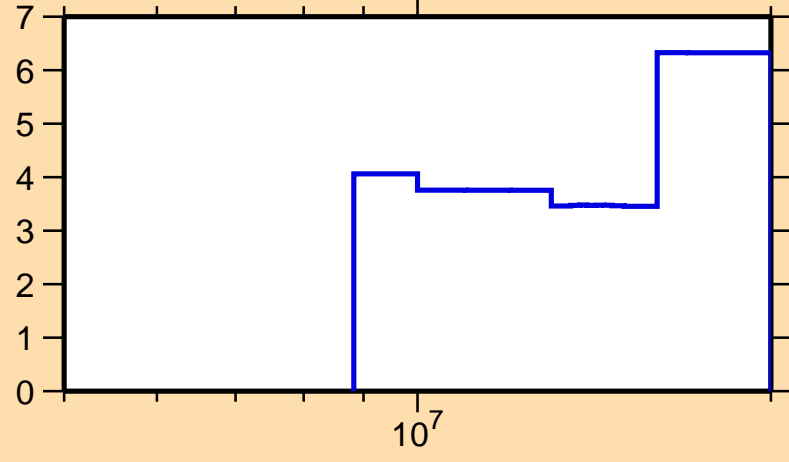
\Delta\sigma/\sigma vs. E for ^{133}\text{Nd}(n,\text{tot.})
