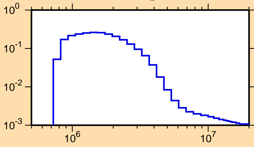
\sigma vs. E for ^{134}\text{Nd}(n,n_2)
