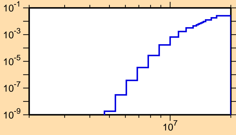
\sigma vs. E for ^{134}\text{Nd}(n,n\alpha)
