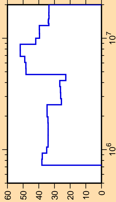
\Delta\sigma/\sigma vs. E for ^{134}\text{Nd}(n,n_2)
