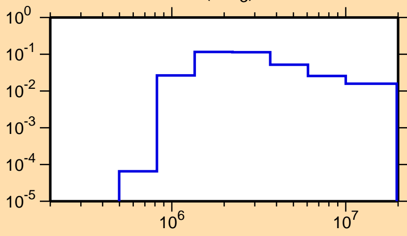
\sigma vs. E for ^{134}\text{Nd}(n,n_3)
