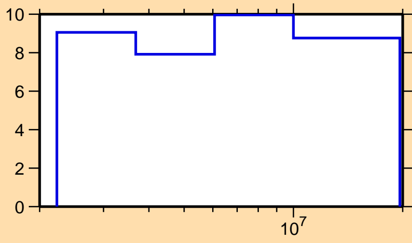
\Delta\sigma/\sigma vs. E for ^{134}\text{Nd}(n,n\text{onel.})
