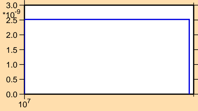
\sigma vs. E for ^{134}\text{Nd} (mt 45)
