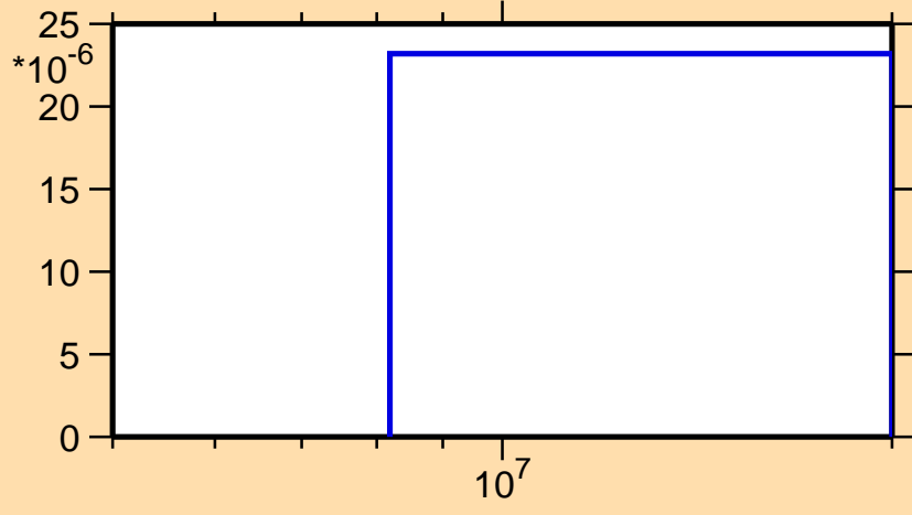
\sigma vs. E for ^{134}\text{Nd}(n,t)
