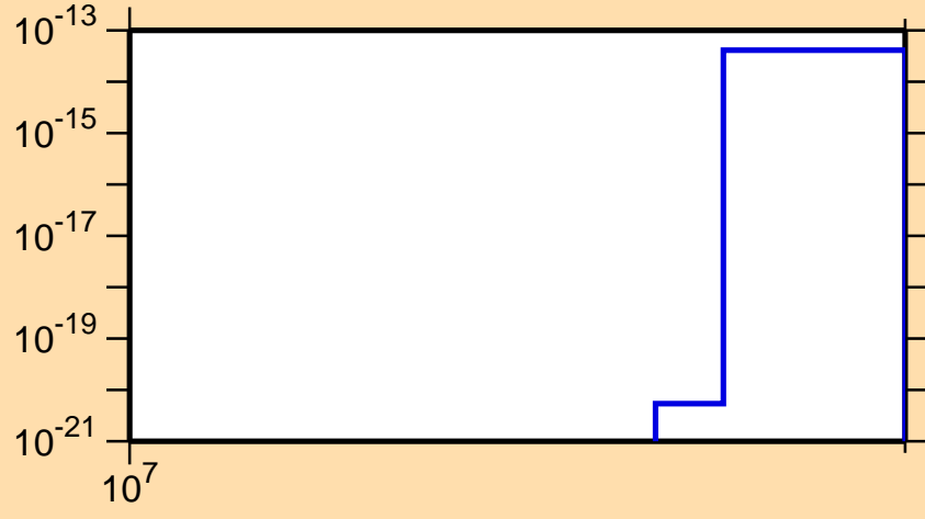
\sigma vs. E for ^{135}\text{Nd}(n,nt)
