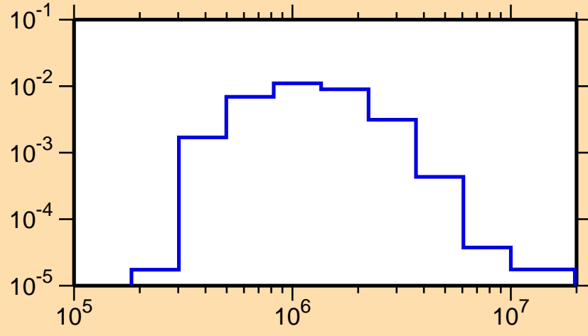
\sigma vs. E for ^{135}\text{Nd}(n,n_4)
