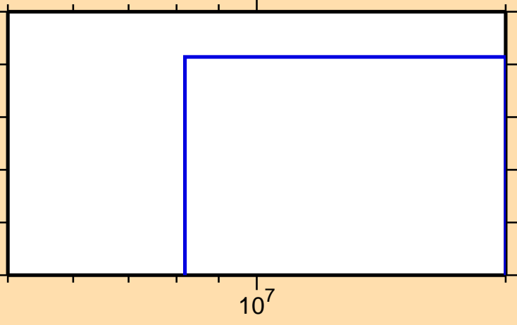
\sigma vs. E for ^{135}\text{Nd}(\text{mt117})
