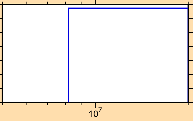
\sigma vs. E for ^{135}\text{Nd}(n,2np)
