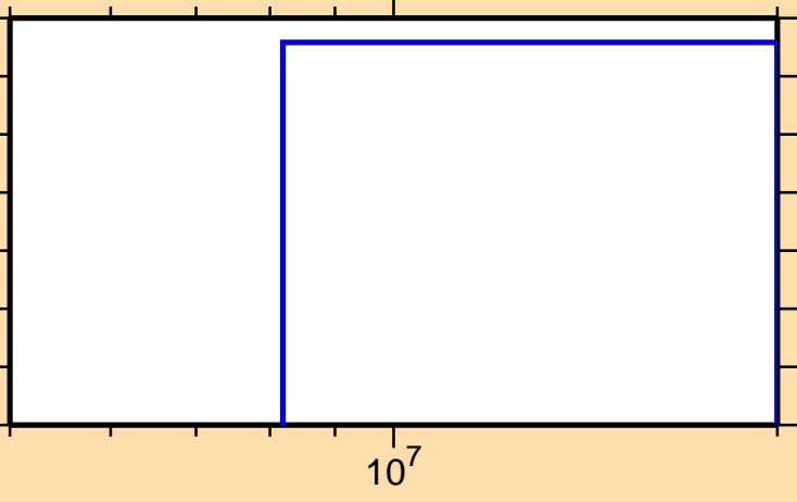
\sigma vs. E for ^{135}\text{Nd}(\text{mt } 45)
