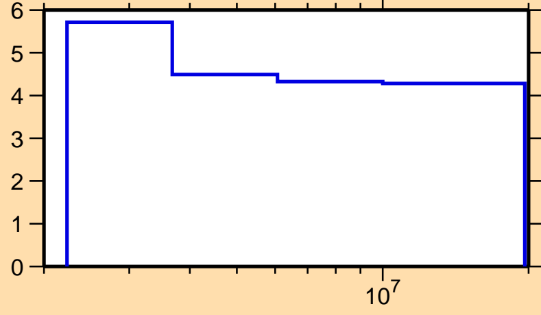
\Delta\sigma/\sigma vs. E for ^{136}\text{Nd}(n,n\text{onel.})
