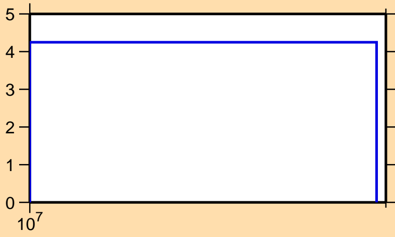
\Delta\sigma/\sigma vs. E for ^{136}\text{Nd}(n,\text{el.})
