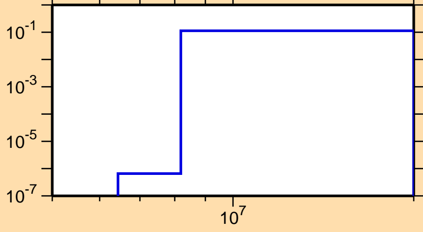
\sigma vs. E for ^{136}\text{Nd}(n,np)
