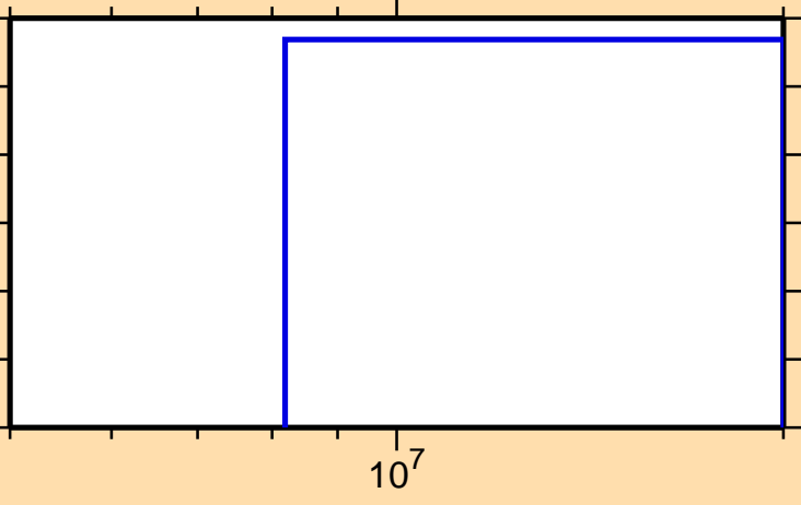
\sigma vs. E for ^{136}\text{Nd}(n,nt)
