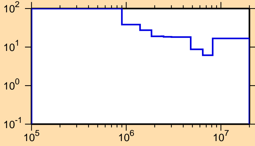
\Delta\sigma/\sigma vs. E for ^{136}\text{Nd}(n,\text{inel.})
