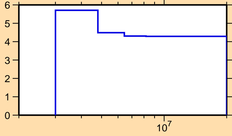
\Delta\sigma/\sigma vs. E for ^{136}\text{Nd}(n,\text{nonel.})
