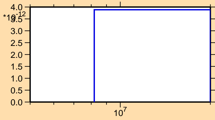
\sigma vs. E for ^{136}\text{Nd}(\text{mt117})
