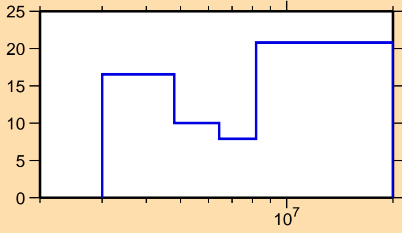
\Delta\sigma/\sigma vs. E for ^{136}\text{Nd}(n,n\text{cont.})
