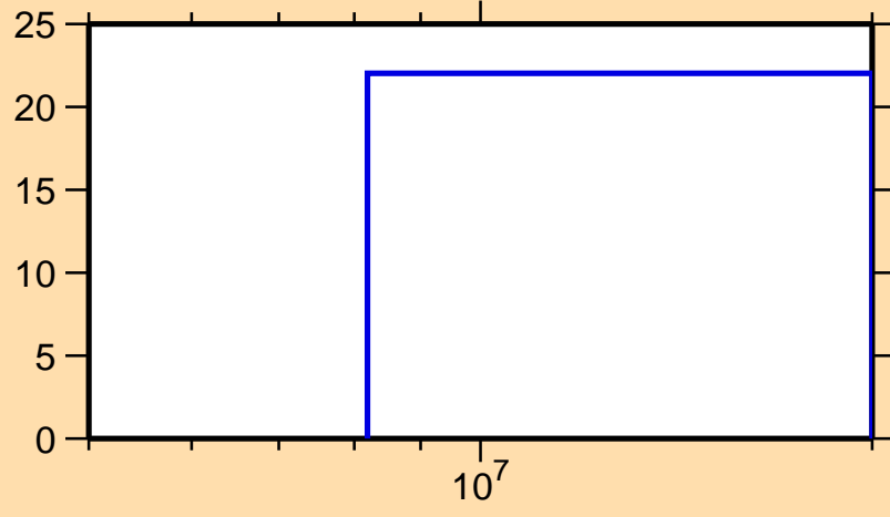
\Delta\sigma/\sigma vs. E for ^{136}\text{Nd}(n,2n)
