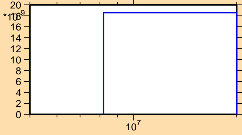
\sigma vs. E for ^{136}\text{Nd}(n,\text{pd})
