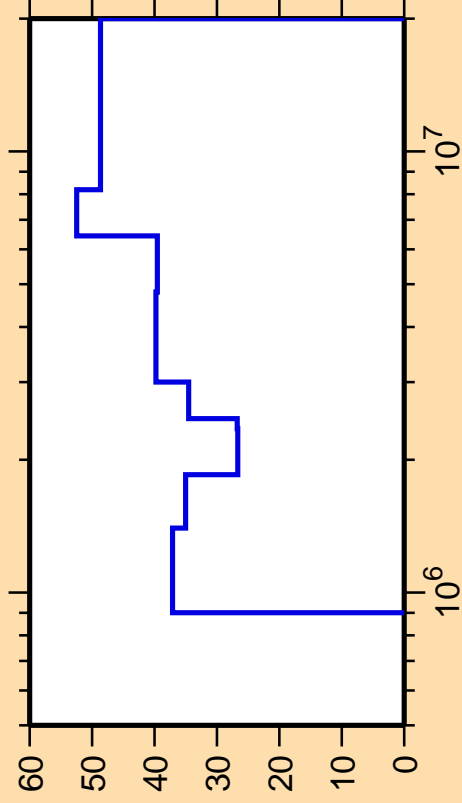
\Delta\sigma/\sigma vs. E for ^{136}\text{Nd}(n,n_4)
