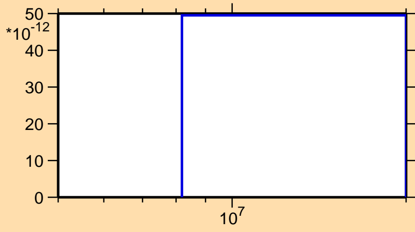
\sigma vs. E for ^{136}\text{Nd}(n,3n)
