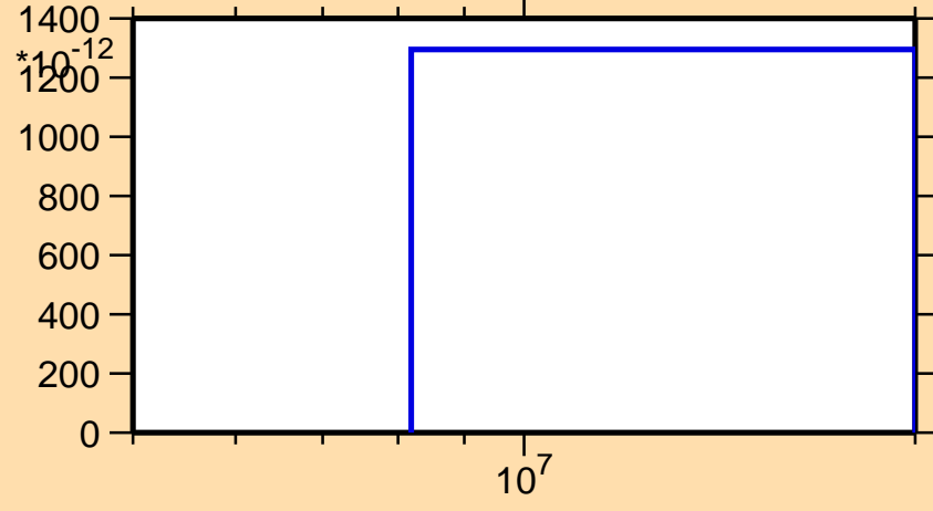
\sigma vs. E for ^{136}\text{Nd}(n,2np)
