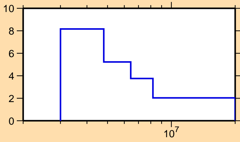
\Delta\sigma/\sigma vs. E for ^{136}\text{Nd}(n,\text{tot.})
