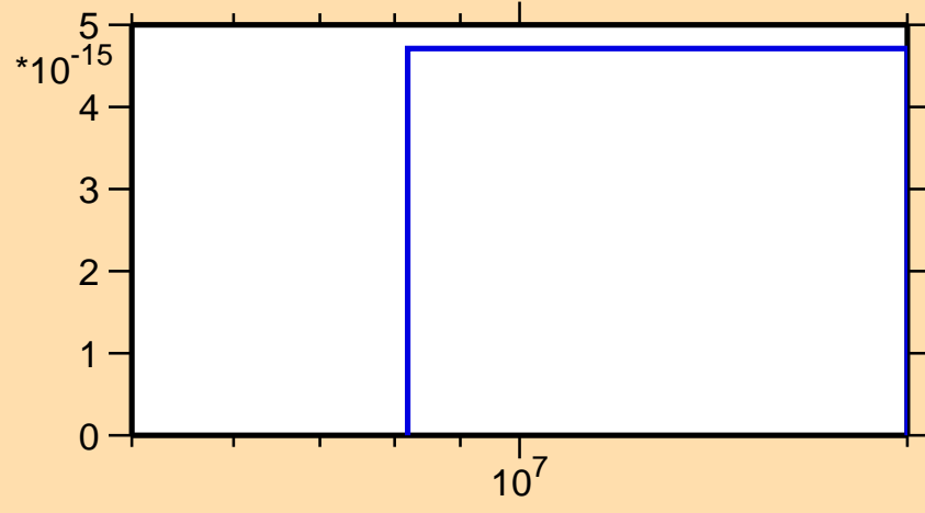
\sigma vs. E for ^{136}\text{Nd}(\text{mt } 34)
