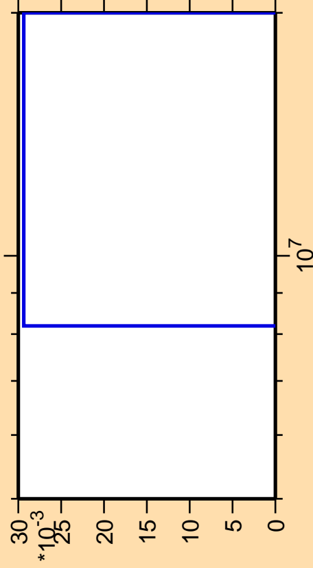
\Delta\sigma/\sigma vs. E for ^{136}\text{Nd}(\text{mt } 34)
