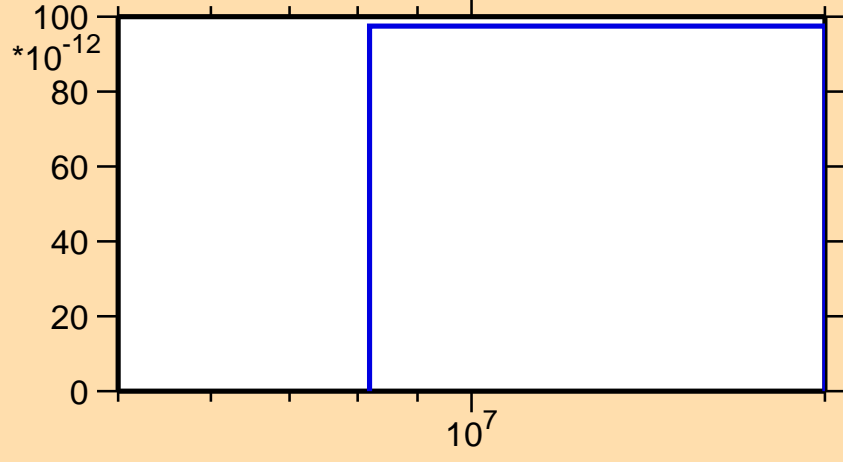
\sigma vs. E for ^{136}\text{Nd}(\text{mt } 45)
