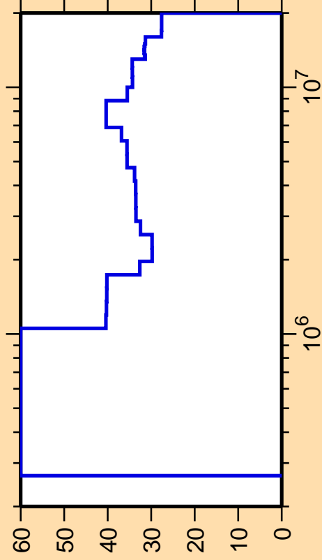
\Delta\sigma/\sigma vs. E for ^{137}\text{Nd}(n,n_2)
