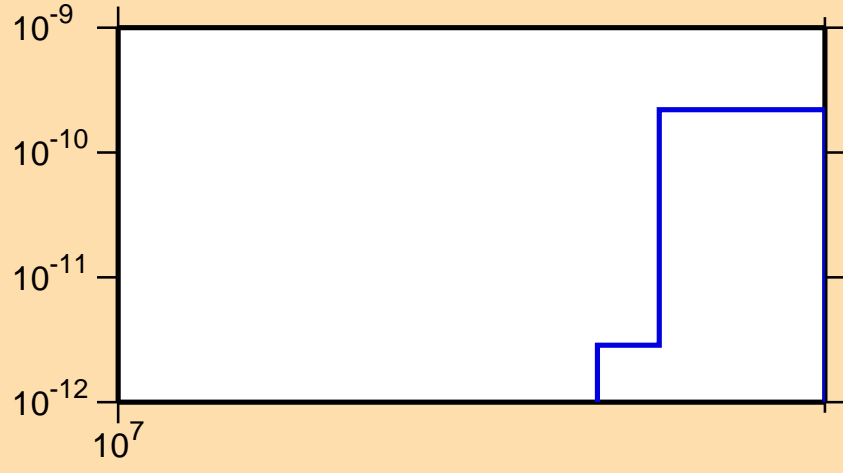
\sigma vs. E for ^{137}\text{Nd} (mt 45)
