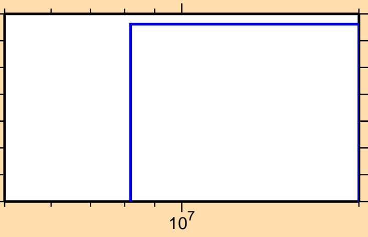
\sigma vs. E for ^{137}\text{Nd}(n,\text{He}3)
