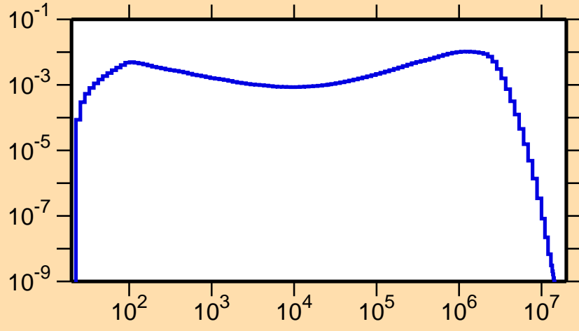
\sigma vs. E for ^{137}\text{Nd}(n,n_3)
