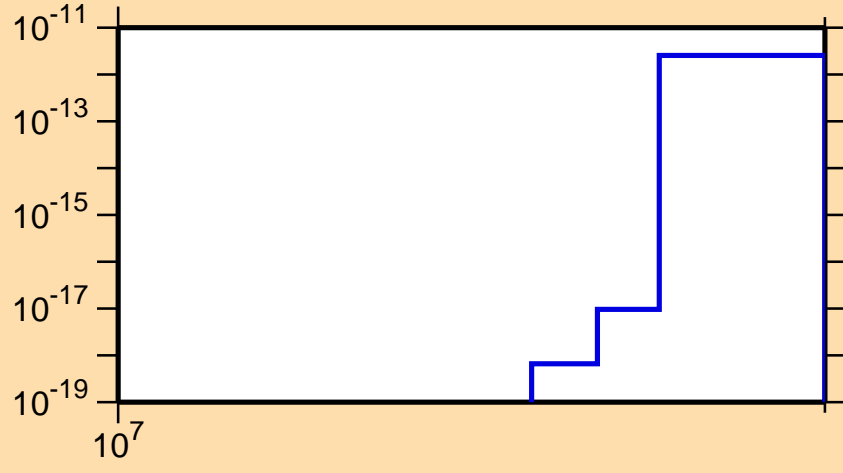
\sigma vs. E for ^{137}\text{Nd}(n,\text{nt})
