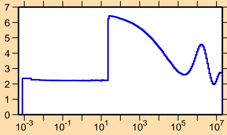
\sigma vs. E for ^{137}\text{Nd}(n,\text{el.})
