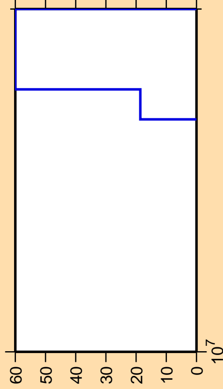
\Delta\sigma/\sigma vs. E for ^{137}\text{Nd} (mt 45)
