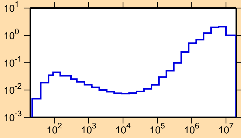
\sigma vs. E for ^{137}\text{Nd}(n,\text{inel.})
