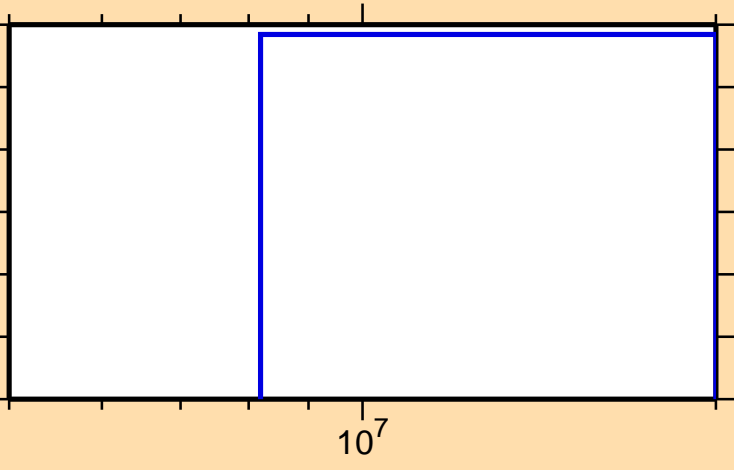
\sigma vs. E for ^{137}\text{Nd}(n,t)
