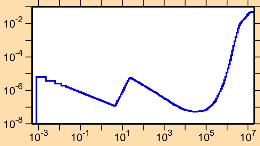
\sigma vs. E for ^{138}\text{Nd}(n,p)
