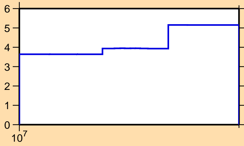
\Delta\sigma/\sigma vs. E for ^{138}\text{Nd}(n,\text{el.})
