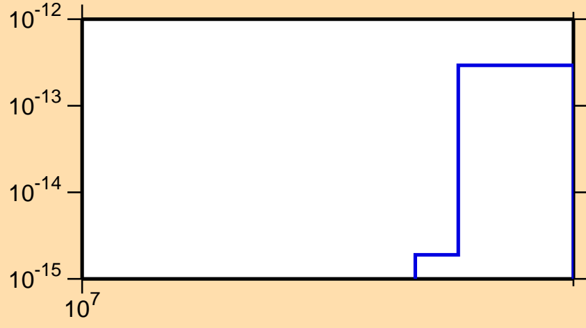
\sigma vs. E for ^{138}\text{Nd}(n,nt)
