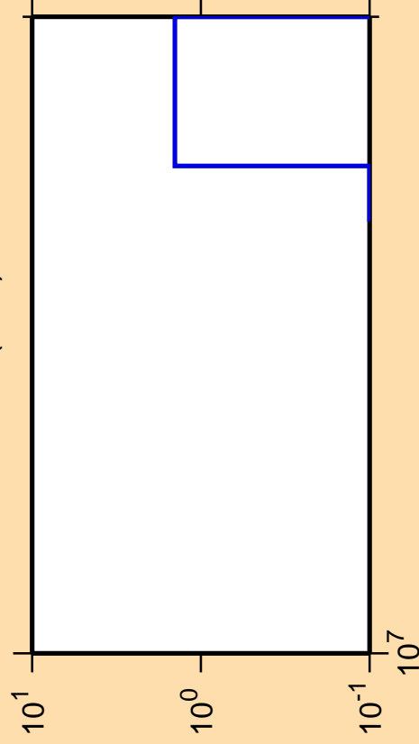
\Delta\sigma/\sigma vs. E for ^{138}\text{Nd}(n,nt)
