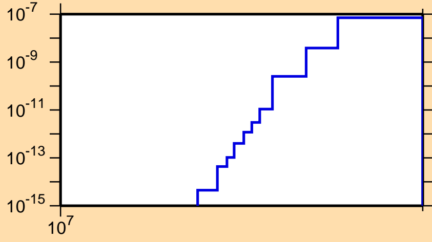
\sigma vs. E for ^{138}\text{Nd}(n,\text{pd})
