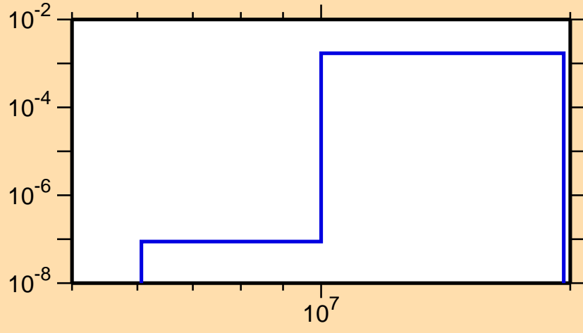
\sigma vs. E for ^{138}\text{Nd}(n,d)
