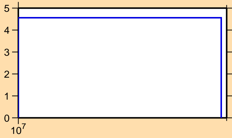
\Delta\sigma/\sigma vs. E for ^{138}\text{Nd}(n,\text{inel.})
