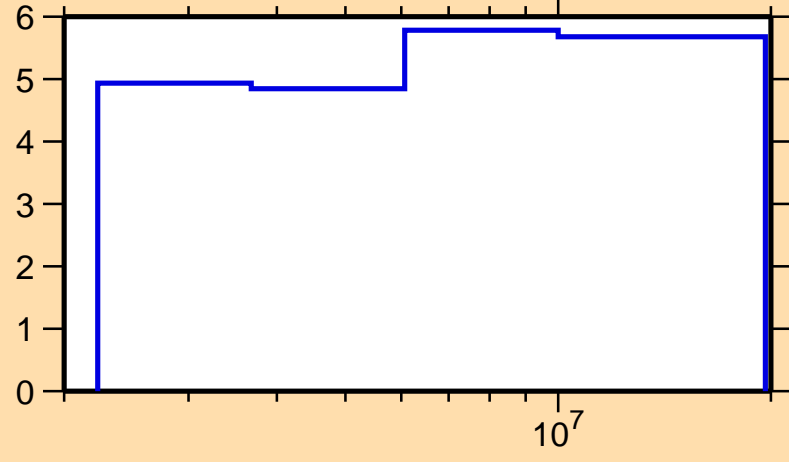
\Delta\sigma/\sigma vs. E for ^{138}\text{Nd}(n,n\text{onel.})
