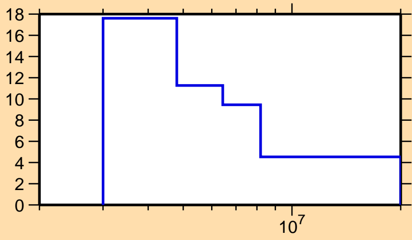
\Delta\sigma/\sigma vs. E for ^{138}\text{Nd}(n,n\text{cont.})
