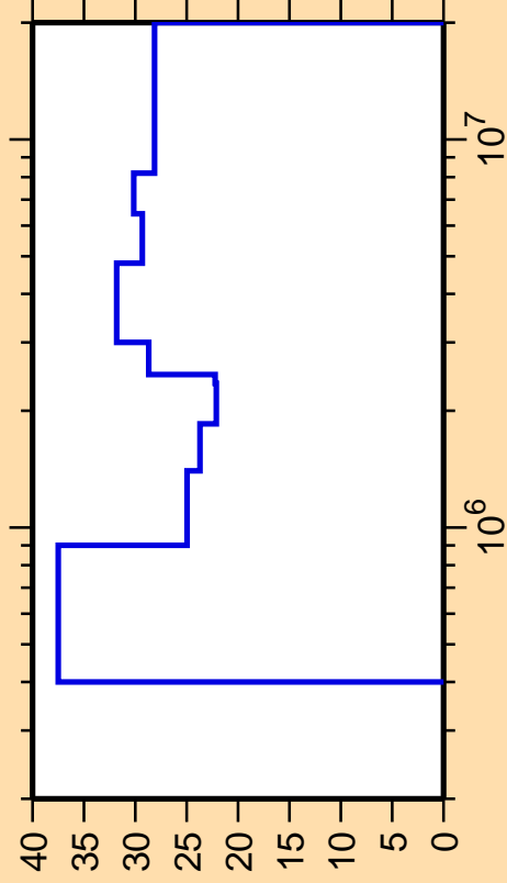
\Delta\sigma/\sigma vs. E for ^{138}\text{Nd}(n,n_1)
