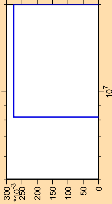
\Delta\sigma/\sigma vs. E for ^{138}\text{Nd}(\text{mt117})
