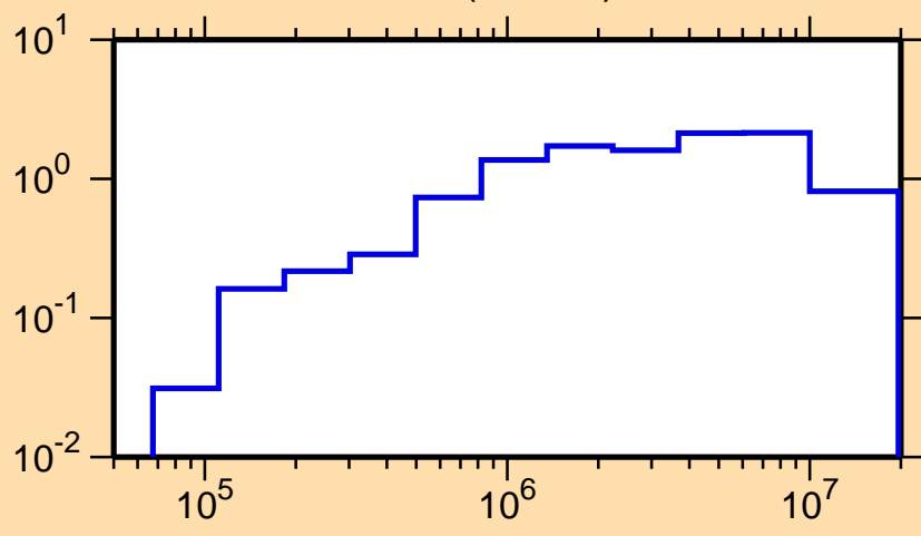
\sigma vs. E for ^{139}\text{Nd}(n,\text{inel.})
