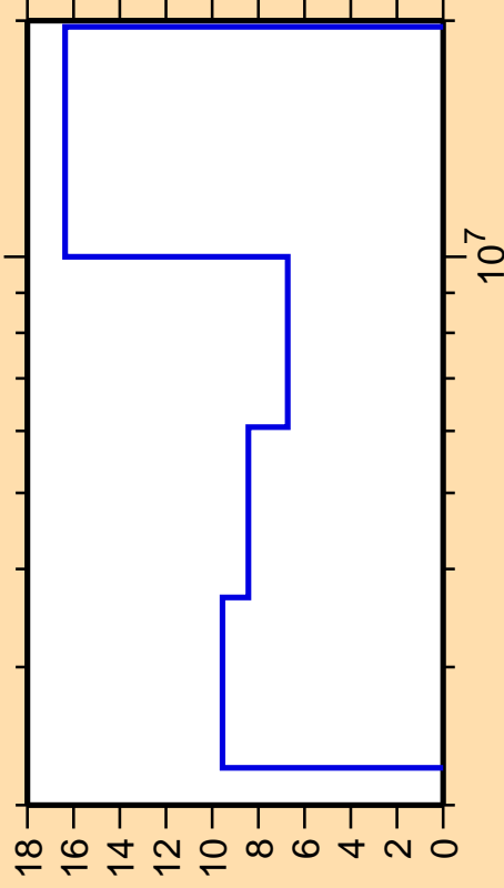
\Delta\sigma/\sigma vs. E for ^{139}\text{Nd}(n,n\text{cont.})
