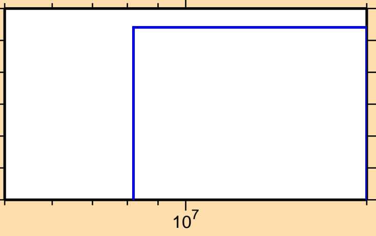
\sigma vs. E for ^{139}\text{Nd}(n,\text{nd})
