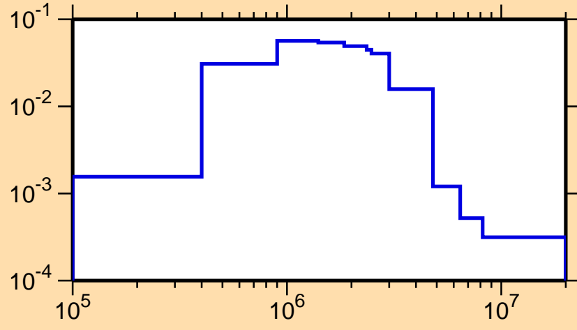
\sigma vs. E for ^{139}\text{Nd}(n,n_2)
