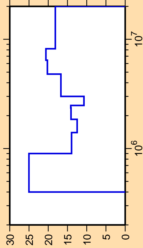
\Delta\sigma/\sigma vs. E for ^{139}\text{Nd}(n,n_4)
