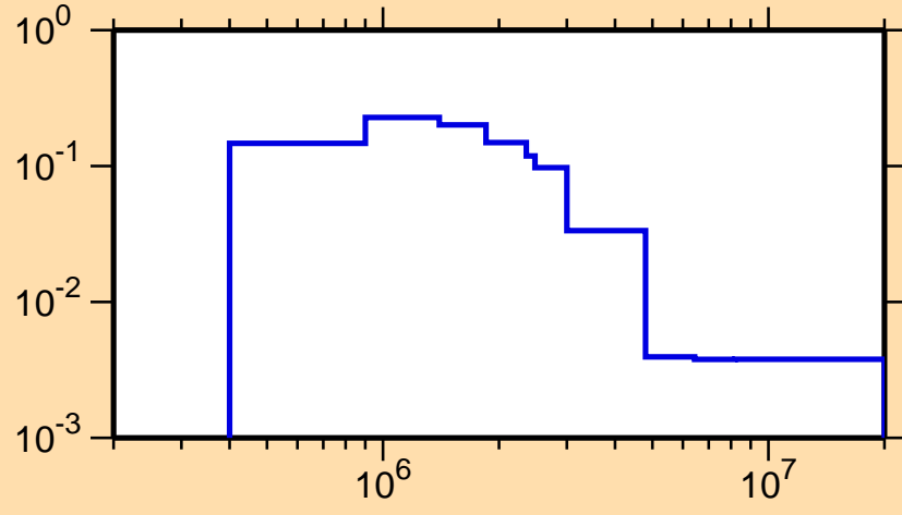
\sigma vs. E for ^{139}\text{Nd}(n,n_4)
