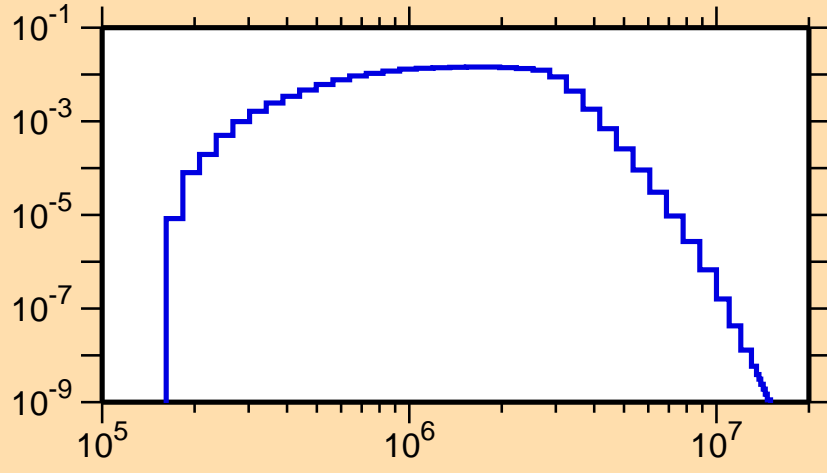
\sigma vs. E for ^{139}\text{Nd}(n,n_3)
