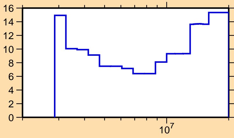
\Delta\sigma/\sigma vs. E for ^{140}\text{Nd}(n,n\text{cont.})
