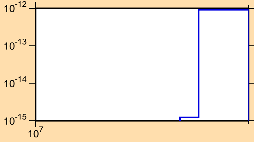
\sigma vs. E for ^{140}\text{Nd} (mt 45)
