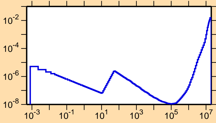
\sigma vs. E for ^{140}\text{Nd}(n,\alpha)
