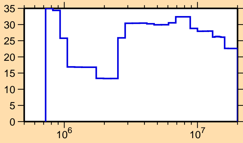
\Delta\sigma/\sigma vs. E for ^{140}\text{Nd}(n,n_1)
