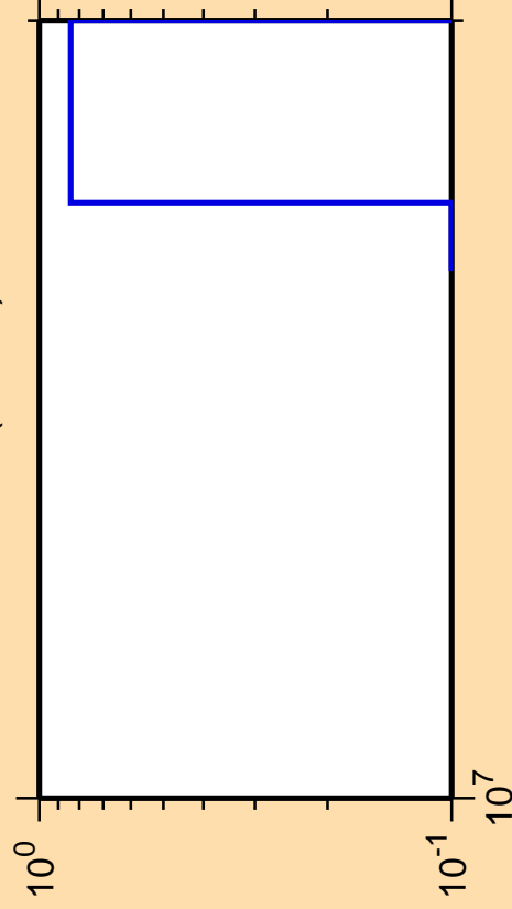
\Delta\sigma/\sigma vs. E for ^{140}\text{Nd} (mt 45)
