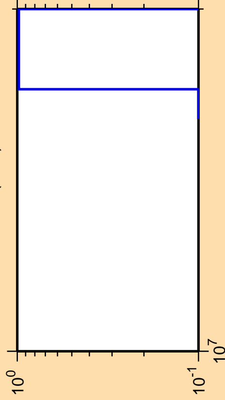
\Delta\sigma/\sigma vs. E for ^{140}\text{Nd}(n,nt)
