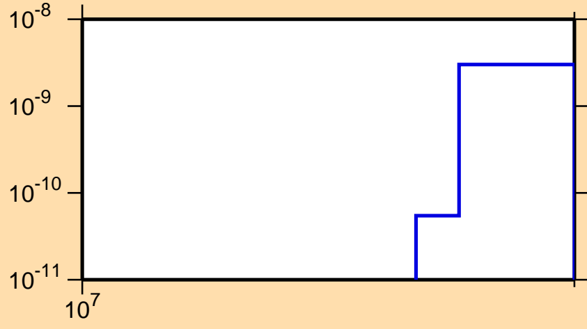
\sigma vs. E for ^{140}\text{Nd}(n,\text{pd})
