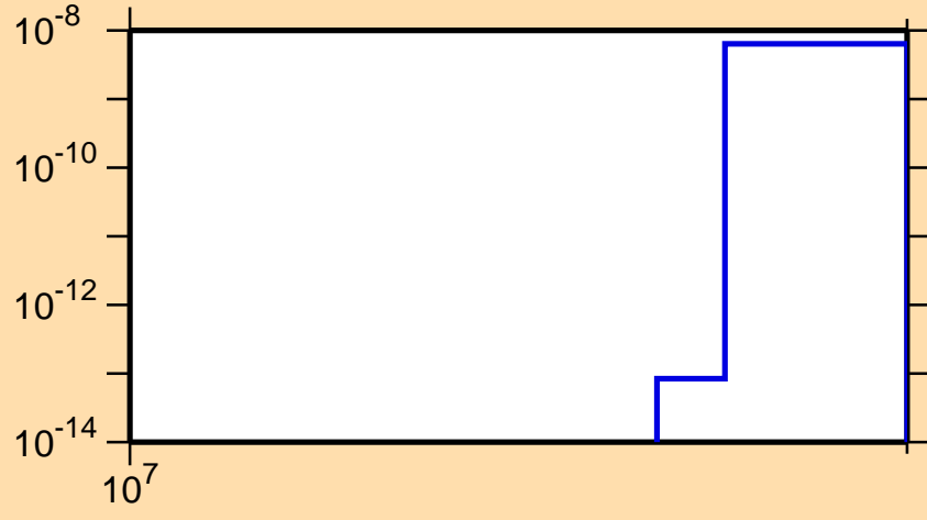
\sigma vs. E for ^{140}\text{Nd}(n,\text{nd})
