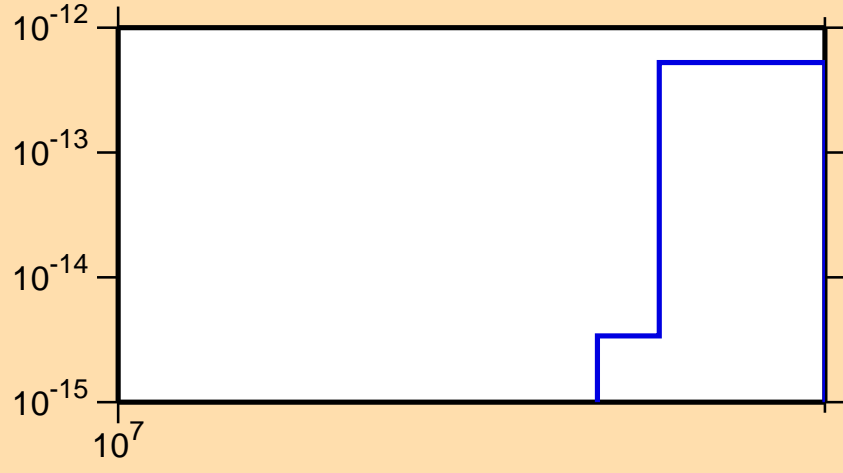
\sigma vs. E for ^{140}\text{Nd}(\text{mt117})
