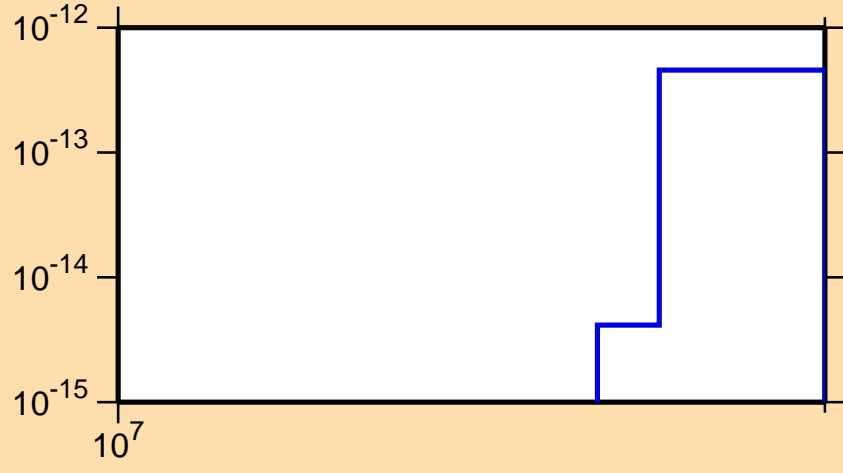
\sigma vs. E for ^{140}\text{Nd}(n,nt)
