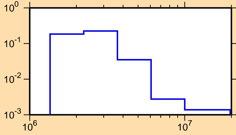
\sigma vs. E for ^{140}\text{Nd}(n,n_4)
