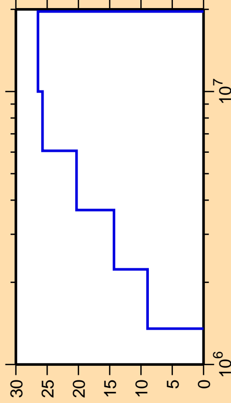
\Delta\sigma/\sigma vs. E for ^{140}\text{Nd}(n,n_4)
