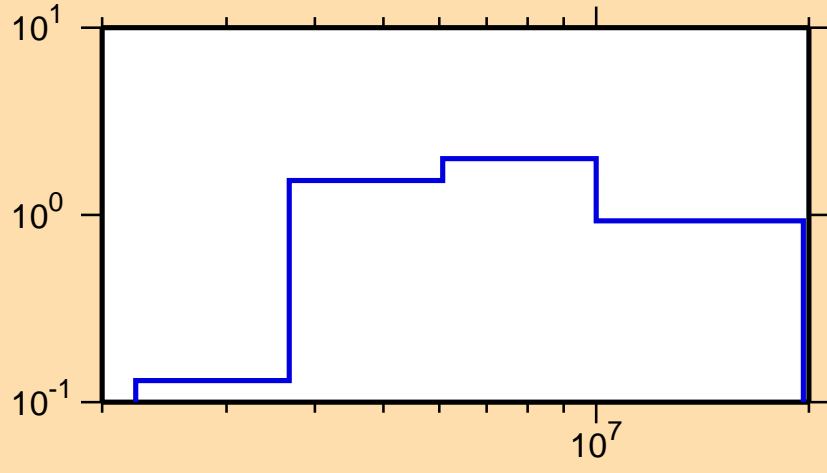
\sigma vs. E for ^{140}\text{Nd}(n,n\text{cont.})
