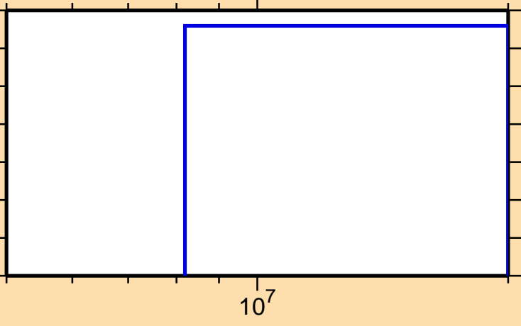
\sigma vs. E for ^{140}\text{Nd}(n,p\alpha)
