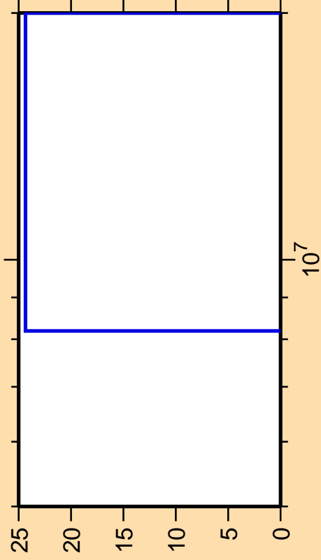
\Delta\sigma/\sigma vs. E for ^{140}\text{Nd}(n,pd)
