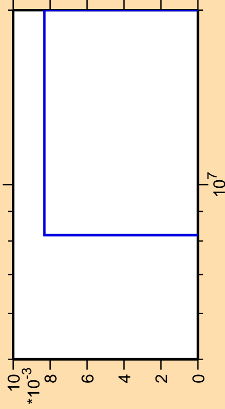
\Delta\sigma/\sigma vs. E for ^{140}\text{Nd}(n,nt)
