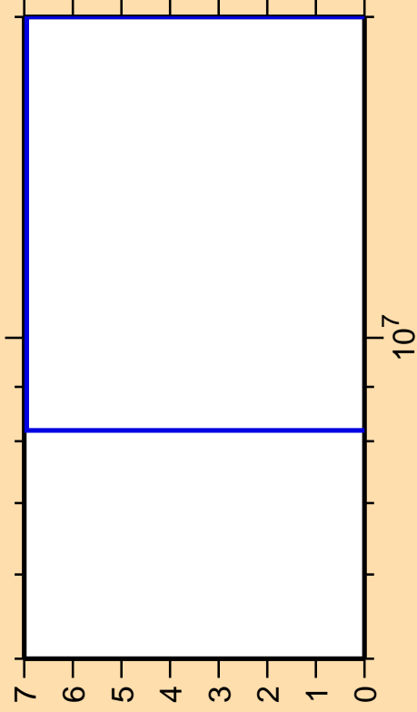
\Delta\sigma/\sigma vs. E for ^{140}\text{Nd}(n,2n)
