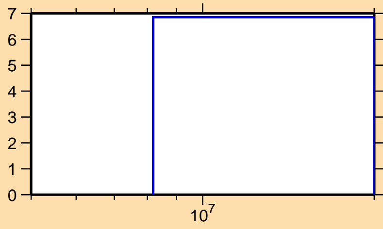
\Delta\sigma/\sigma vs. E for ^{140}\text{Nd}(n,\text{inel.})
