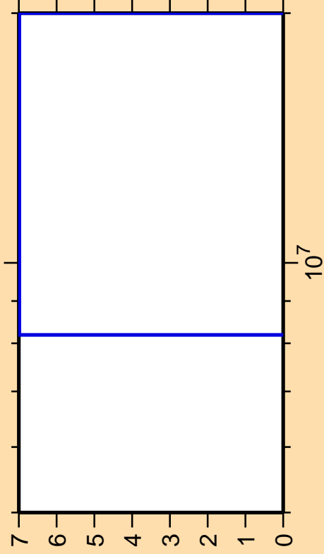
\Delta\sigma/\sigma vs. E for ^{140}\text{Nd}(n,2np)
