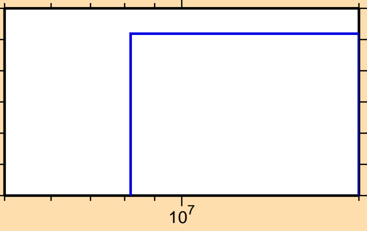
\sigma vs. E for ^{140}\text{Nd}(n,\text{nd})
