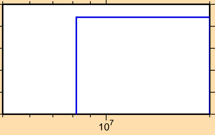
\sigma vs. E for ^{140}\text{Nd}(\text{mt117})
