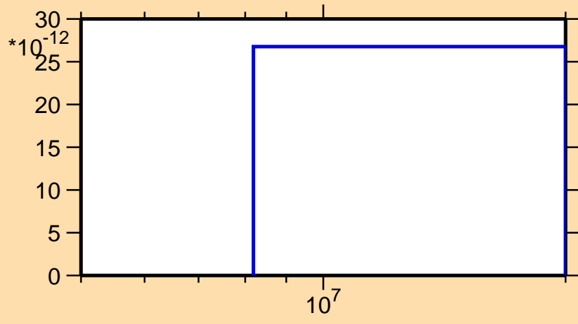
\sigma vs. E for ^{140}\text{Nd}(n,pd)
