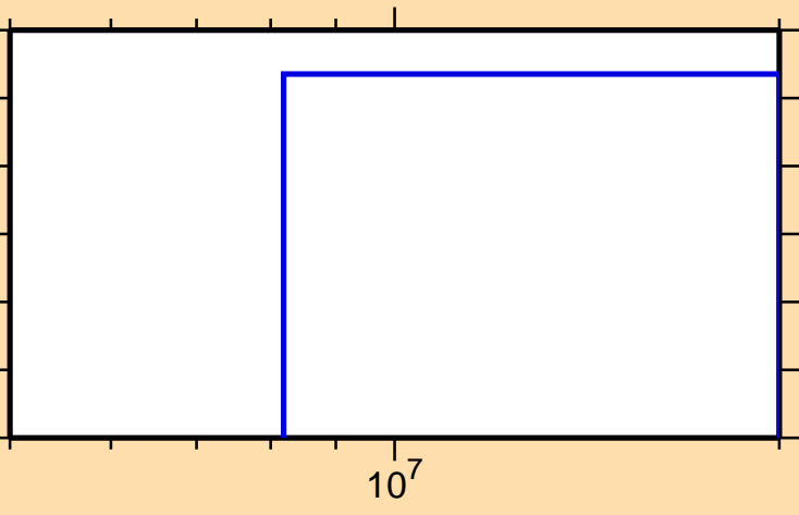
\sigma vs. E for ^{140}\text{Nd}(n,pd)
