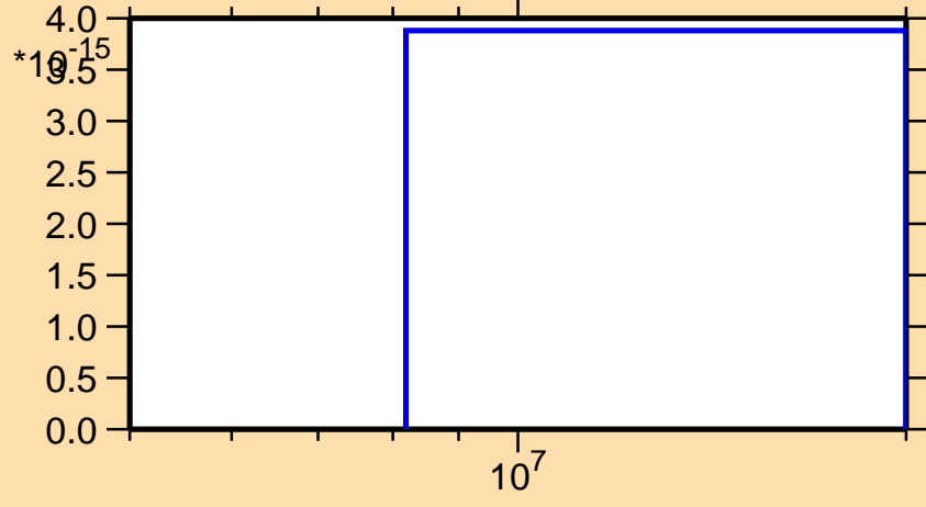
\sigma vs. E for ^{140}\text{Nd}(n,nt)
