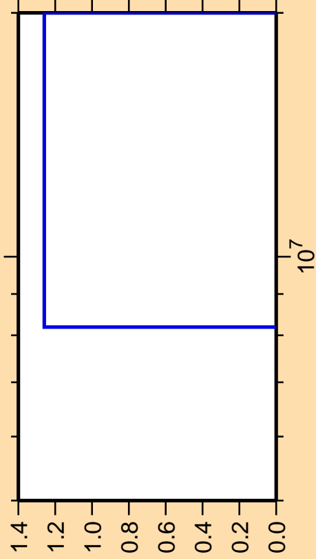
\Delta\sigma/\sigma vs. E for ^{141}\text{Nd}(n,pd)
