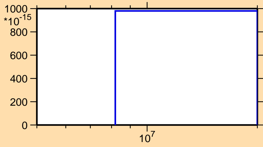
\sigma vs. E for ^{141}\text{Nd}(n,pd)
