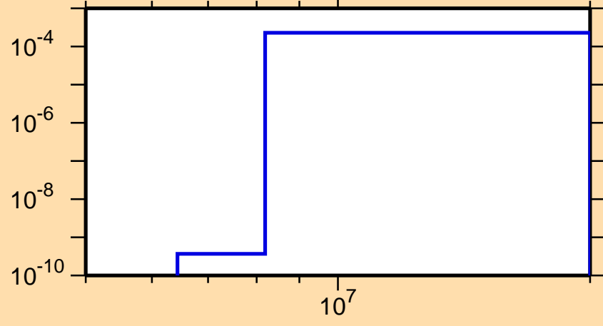
\sigma vs. E for ^{141}\text{Nd}(n,n\alpha)
