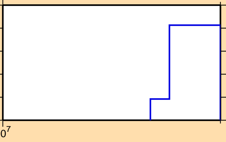
\sigma vs. E for ^{141}\text{Nd} (mt 34)
