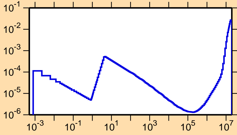
\sigma vs. E for ^{141}\text{Nd}(n,\alpha)
