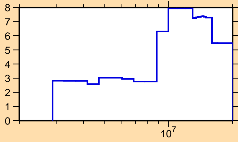
\Delta\sigma/\sigma vs. E for ^{142}\text{Nd}(n,\text{inel.})
