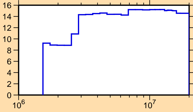
\Delta\sigma/\sigma vs. E for ^{142}\text{Nd}(n,n_1)
