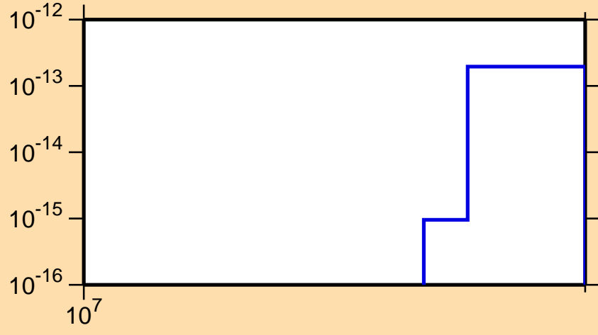
\sigma vs. E for ^{142}\text{Nd}(n,nt)
