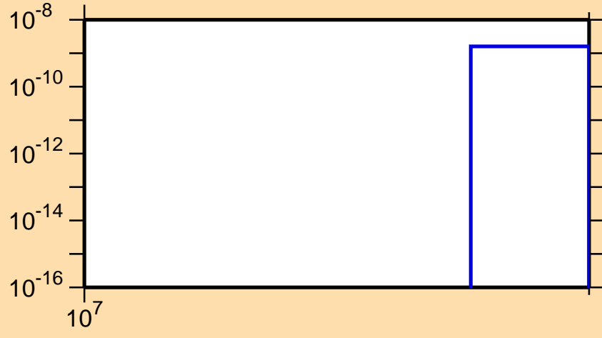
\sigma vs. E for ^{142}\text{Nd}(n,2np)
