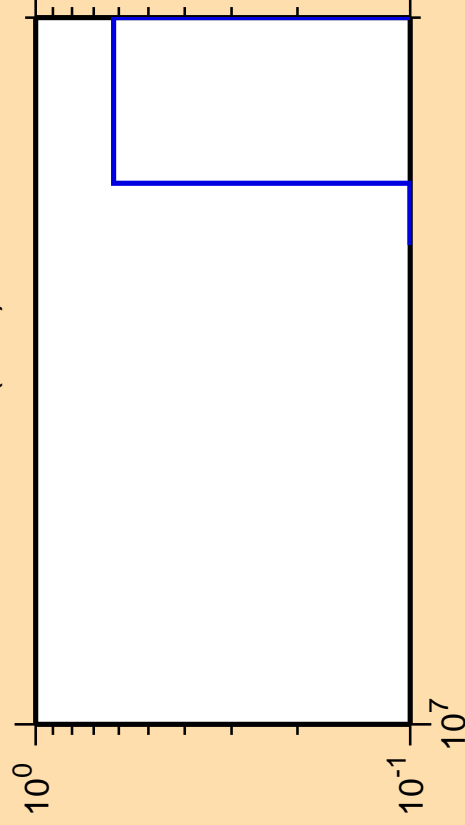
\Delta\sigma/\sigma vs. E for ^{142}\text{Nd}(n,nt)
