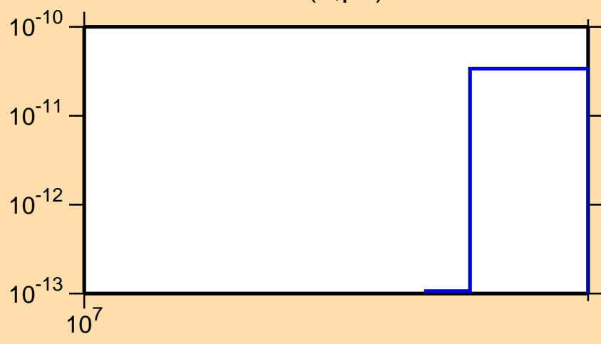
\sigma vs. E for ^{142}\text{Nd}(n,\text{pd})
