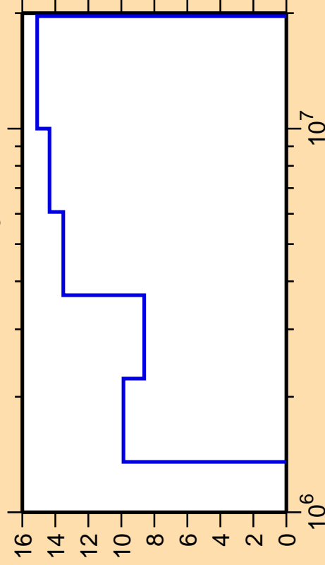
\Delta\sigma/\sigma vs. E for ^{142}\text{Nd}(n,n_3)
