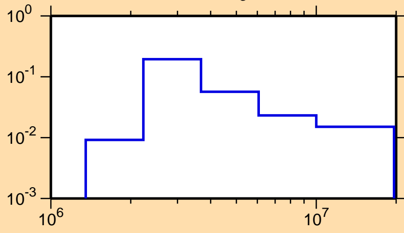
\sigma vs. E for ^{142}\text{Nd}(n,n_3)
