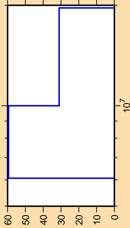
\Delta\sigma/\sigma vs. E for ^{142}\text{Nd}(n,n\alpha)
