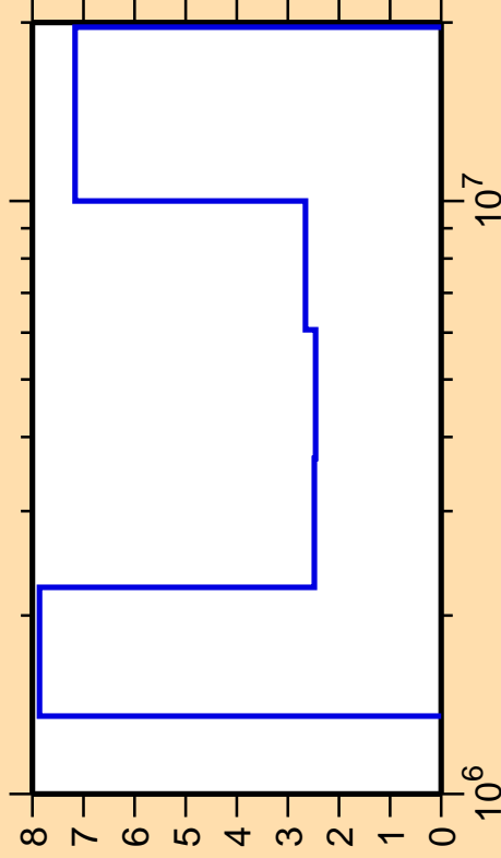
\Delta\sigma/\sigma vs. E for ^{142}\text{Nd}(n,\text{inel.})
