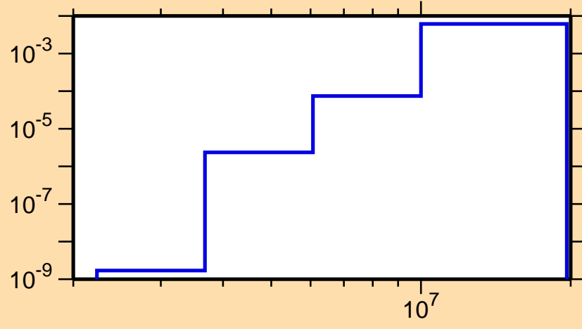
\sigma vs. E for ^{142}\text{Nd}(n,p)
