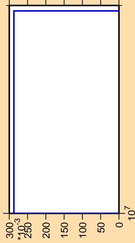
\Delta\sigma/\sigma vs. E for ^{142}\text{Nd}(n,pd)
