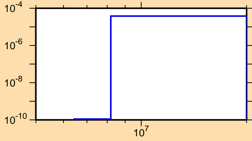
\sigma vs. E for ^{142}\text{Nd}(n,n\alpha)
