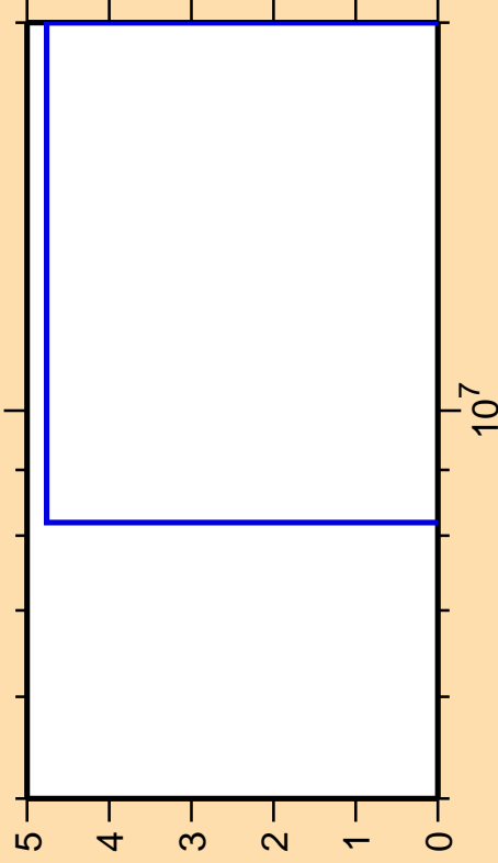
\Delta\sigma/\sigma vs. E for ^{142}\text{Nd}(n,2n)
