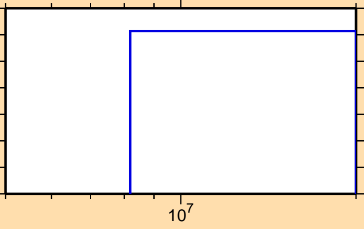
\sigma vs. E for ^{142}\text{Nd}(n,\text{nd})
