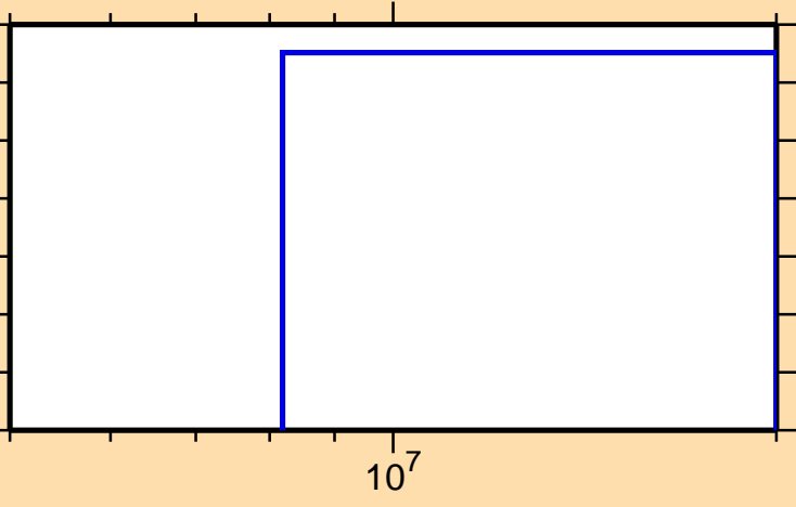
\sigma vs. E for ^{142}\text{Nd}(n,2np)
