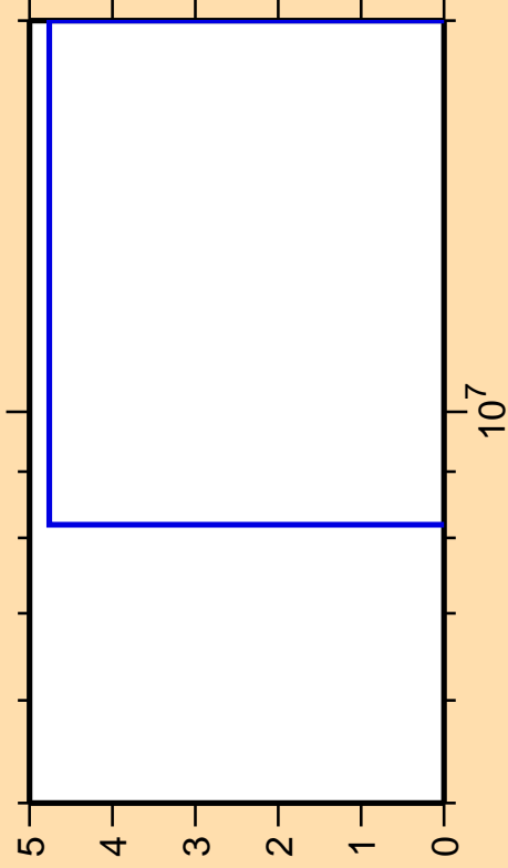
\Delta\sigma/\sigma vs. E for ^{142}\text{Nd}(n,2n)
