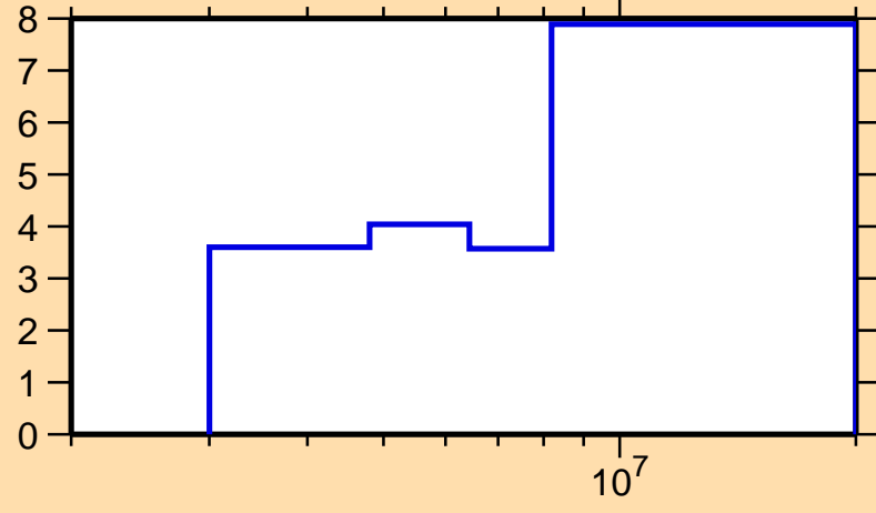
\Delta\sigma/\sigma vs. E for ^{142}\text{Nd}(n,n\text{cont.})
