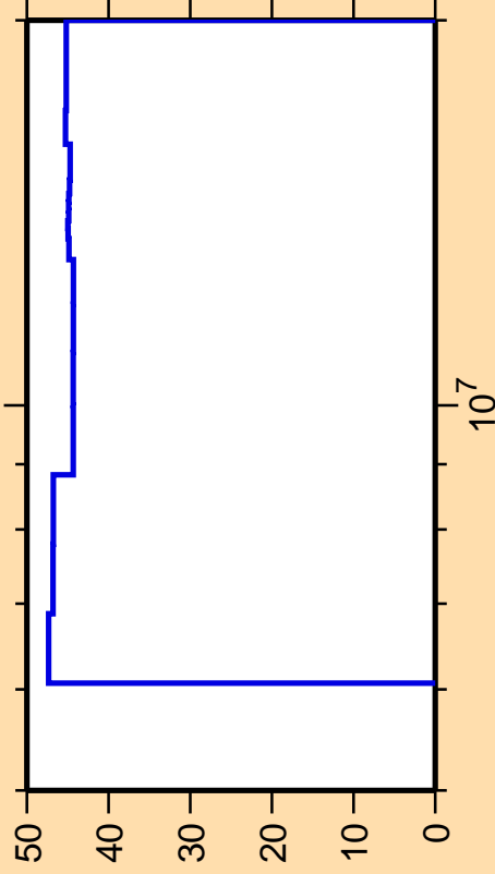
\Delta\sigma/\sigma vs. E for ^{143}\text{Nd}(n,\alpha)
