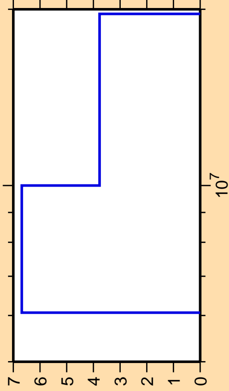
\Delta\sigma/\sigma vs. E for ^{143}\text{Nd}(n,2n)
