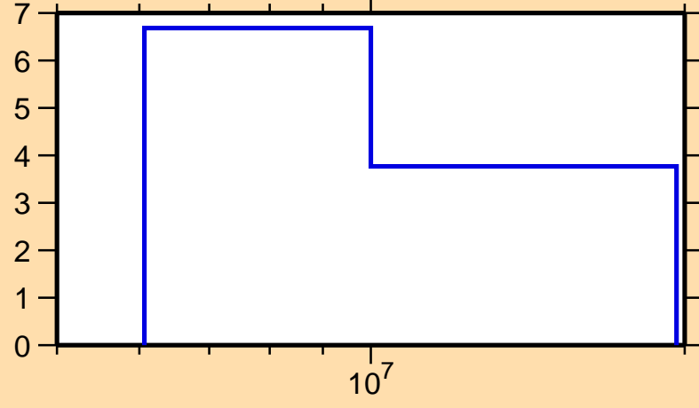
\Delta\sigma/\sigma vs. E for ^{143}\text{Nd}(n,2n)
