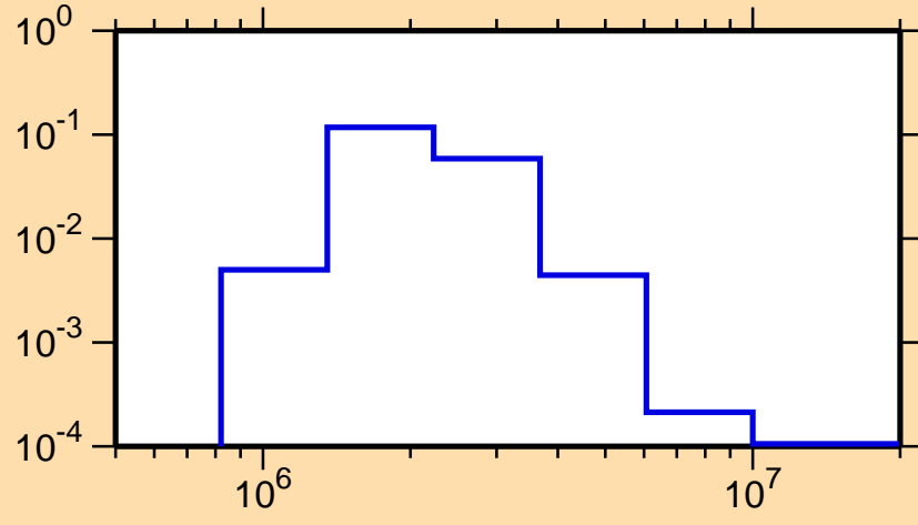
\sigma vs. E for ^{143}\text{Nd}(n,n_2)
