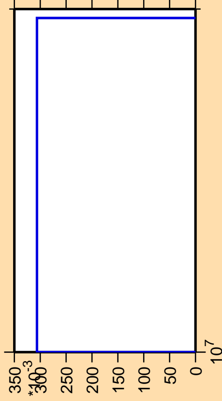
\Delta\sigma/\sigma vs. E for ^{143}\text{Nd}(n,\text{pt})
